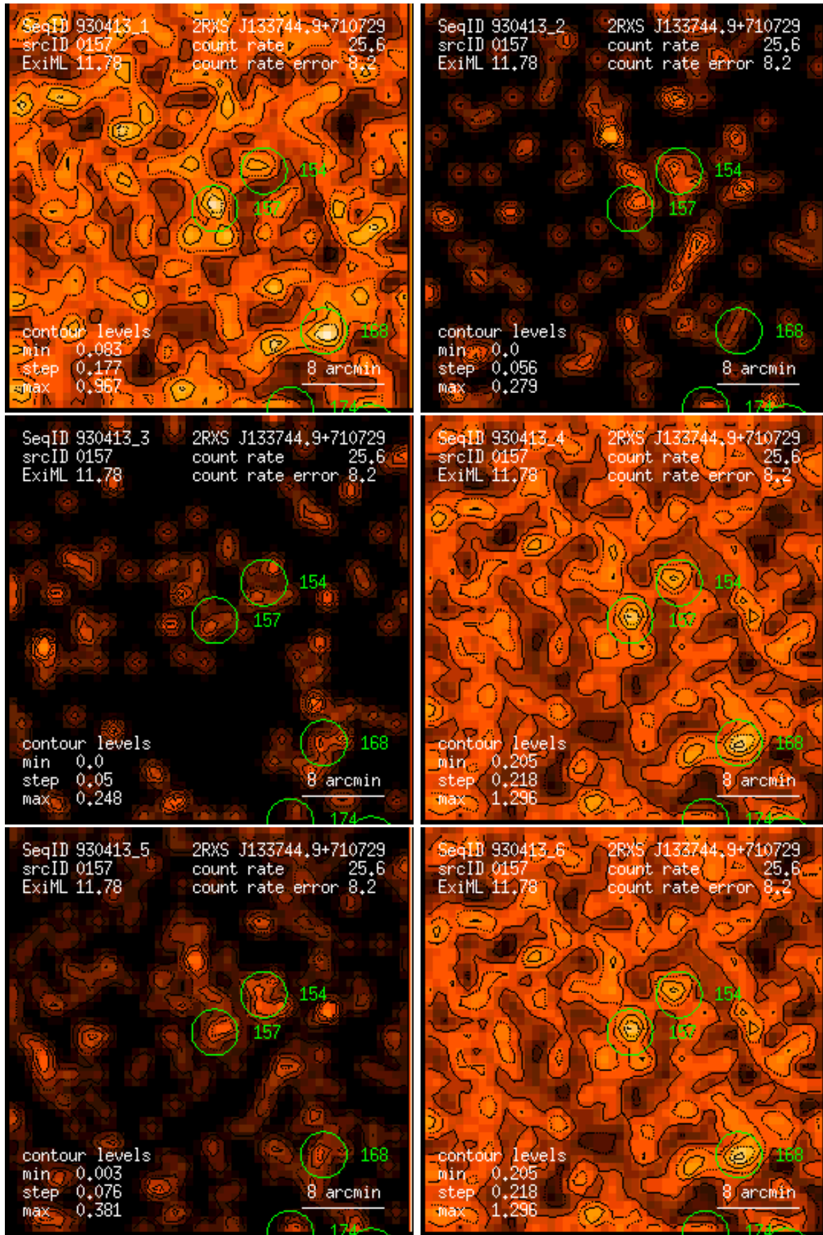
Figure 157: RASS 930413: detection 0157: band rate images, Gaussian filter: (1) PSPC channels 11 – 41, (2) 52 – 90, (3) 91 – 201, (4) 11 – 235, (5) 52 – 201, (6) 11 – 201. Broad band rates in counts/ks. Band rate contour levels in counts/ks/arcmin 2 .
