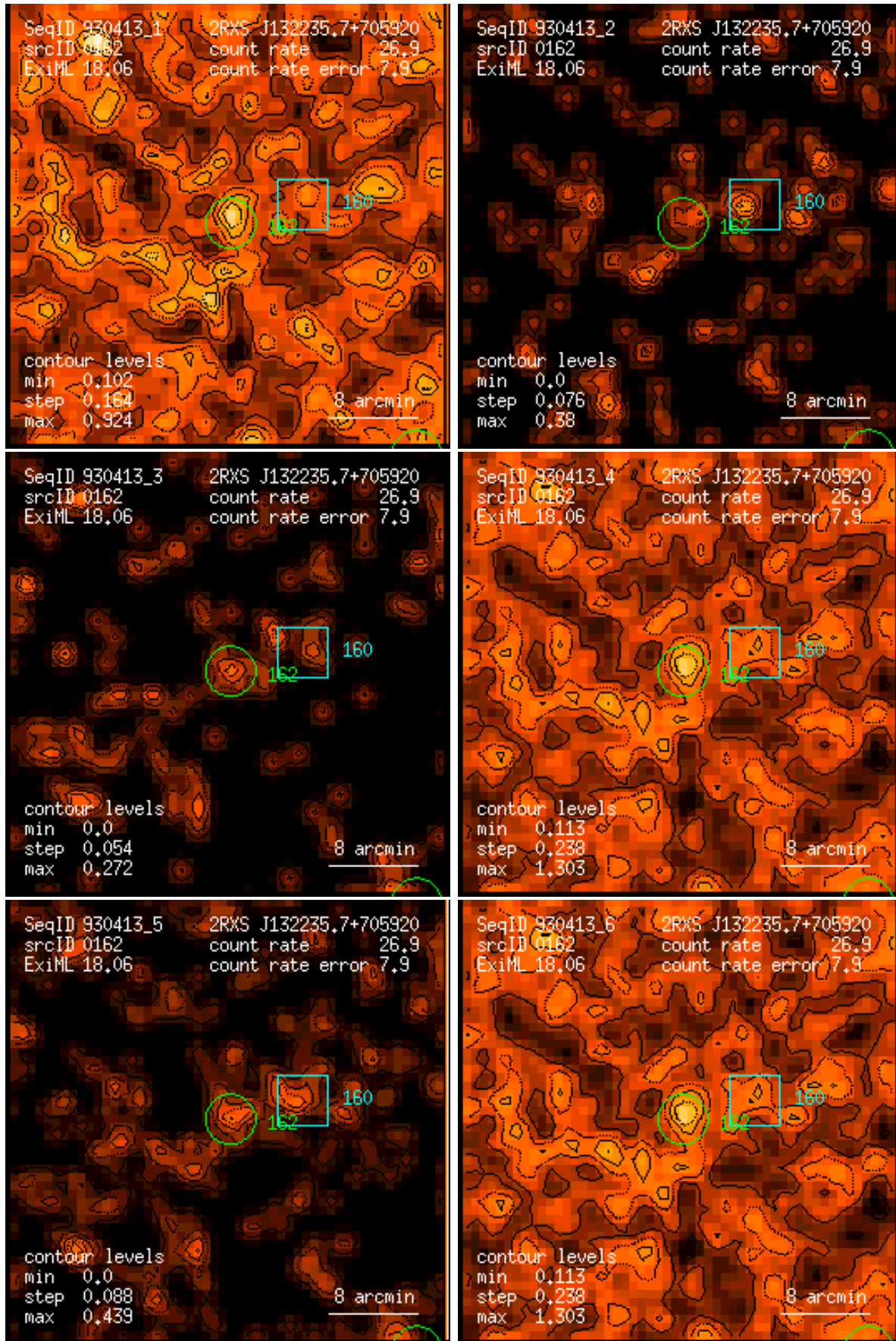
Figure 162: RASS 930413: detection 0162: band rate images, Gaussian filter: (1) PSPC channels 11 – 41, (2) 52 – 90, (3) 91 – 201, (4) 11 – 235, (5) 52 – 201, (6) 11 – 201. Broad band rates in counts/ks. Band rate contour levels in counts/ks/arcmin 2 .
