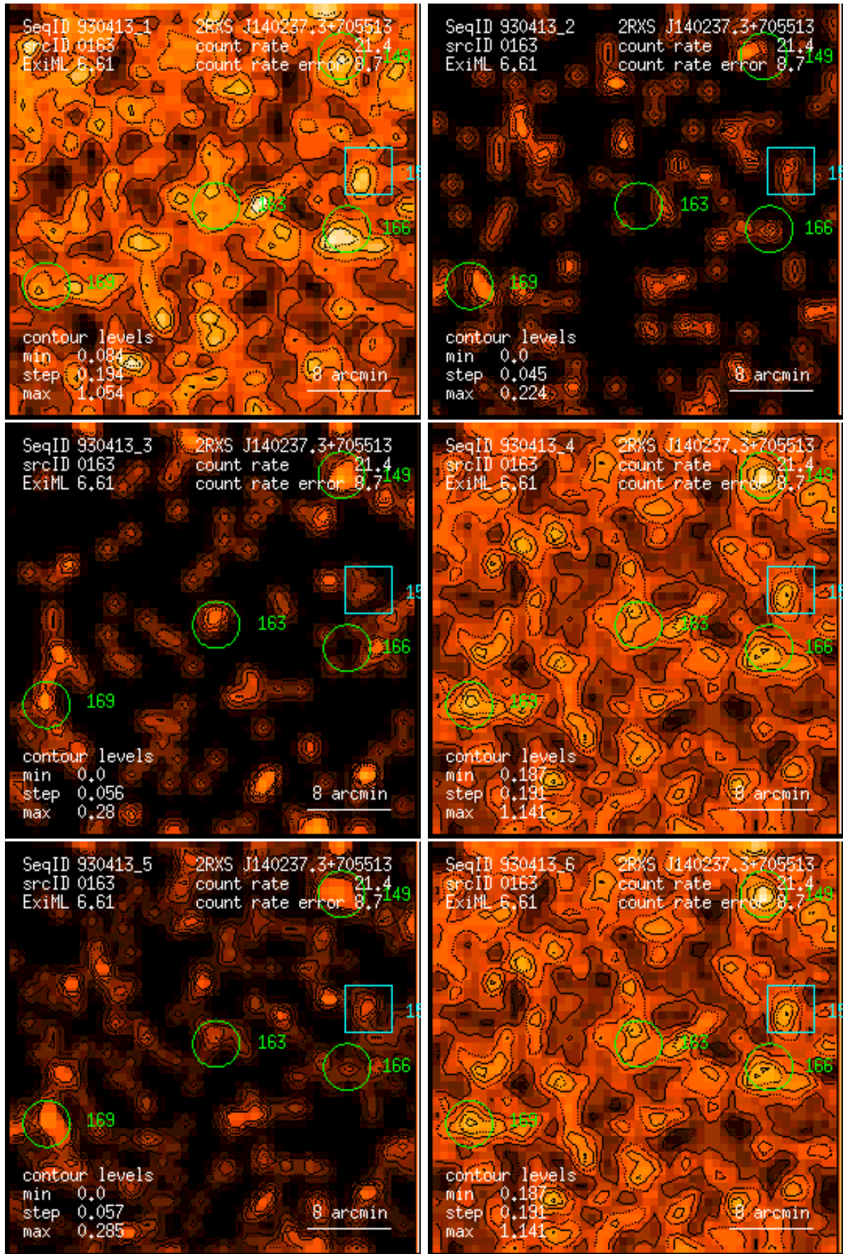
Figure 163: RASS 930413: detection 0163: band rate images, Gaussian filter: (1) PSPC channels 11 – 41, (2) 52 – 90, (3) 91 – 201, (4) 11 – 235, (5) 52 – 201, (6) 11 – 201. Broad band rates in counts/ks. Band rate contour levels in counts/ks/arcmin 2 .
