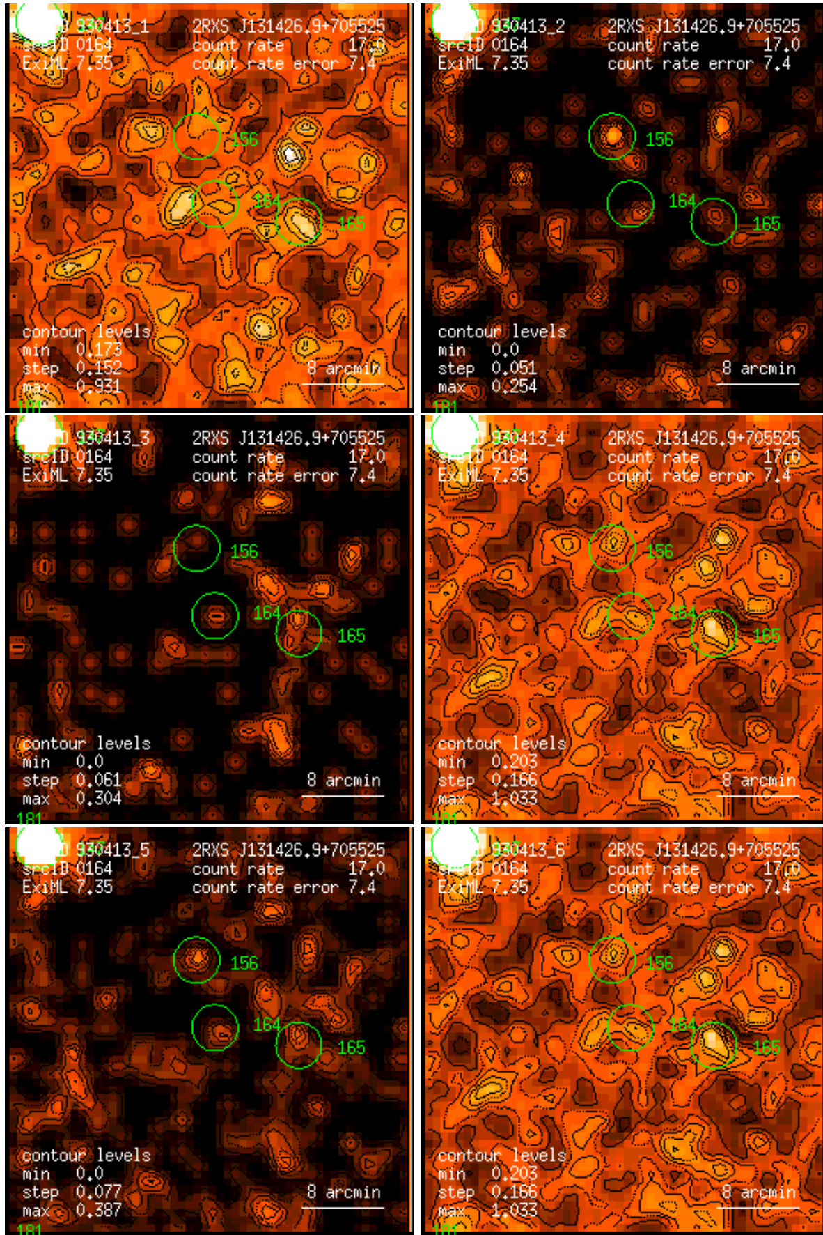
Figure 164: RASS 930413: detection 0164: band rate images, Gaussian filter: (1) PSPC channels 11 – 41, (2) 52 – 90, (3) 91 – 201, (4) 11 – 235, (5) 52 – 201, (6) 11 – 201. Broad band rates in counts/ks. Band rate contour levels in counts/ks/arcmin 2 .
