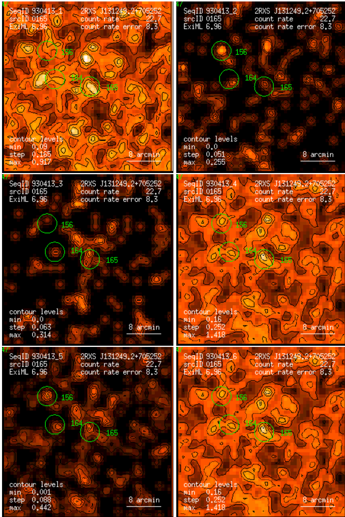
Figure 165: RASS 930413: detection 0165: band rate images, Gaussian filter: (1) PSPC channels 11 – 41, (2) 52 – 90, (3) 91 – 201, (4) 11 – 235, (5) 52 – 201, (6) 11 – 201. Broad band rates in counts/ks. Band rate contour levels in counts/ks/arcmin 2 .
