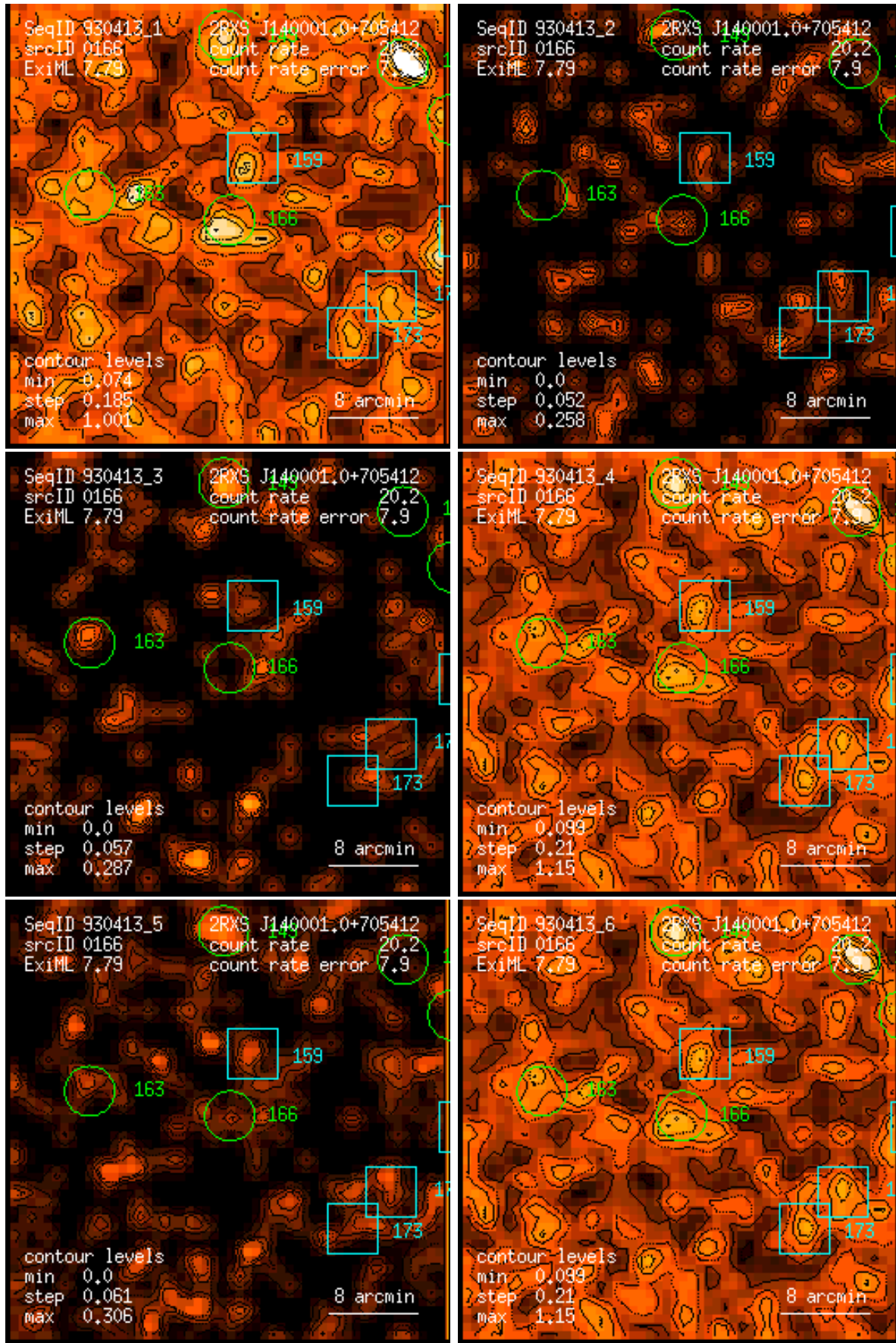
Figure 166: RASS 930413: detection 0166: band rate images, Gaussian filter: (1) PSPC channels 11 – 41, (2) 52 – 90, (3) 91 – 201, (4) 11 – 235, (5) 52 – 201, (6) 11 – 201. Broad band rates in counts/ks. Band rate contour levels in counts/ks/arcmin 2 .
