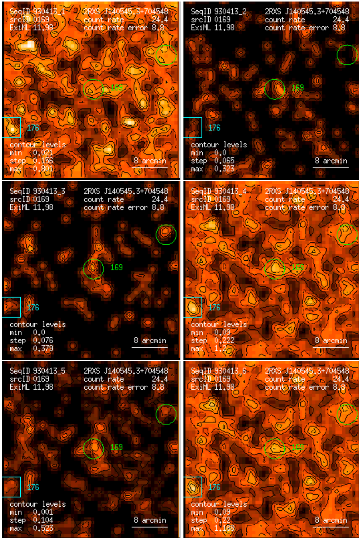
Figure 169: RASS 930413: detection 0169: band rate images, Gaussian filter: (1) PSPC channels 11 – 41, (2) 52 – 90, (3) 91 – 201, (4) 11 – 235, (5) 52 – 201, (6) 11 – 201. Broad band rates in counts/ks. Band rate contour levels in counts/ks/arcmin 2 .
