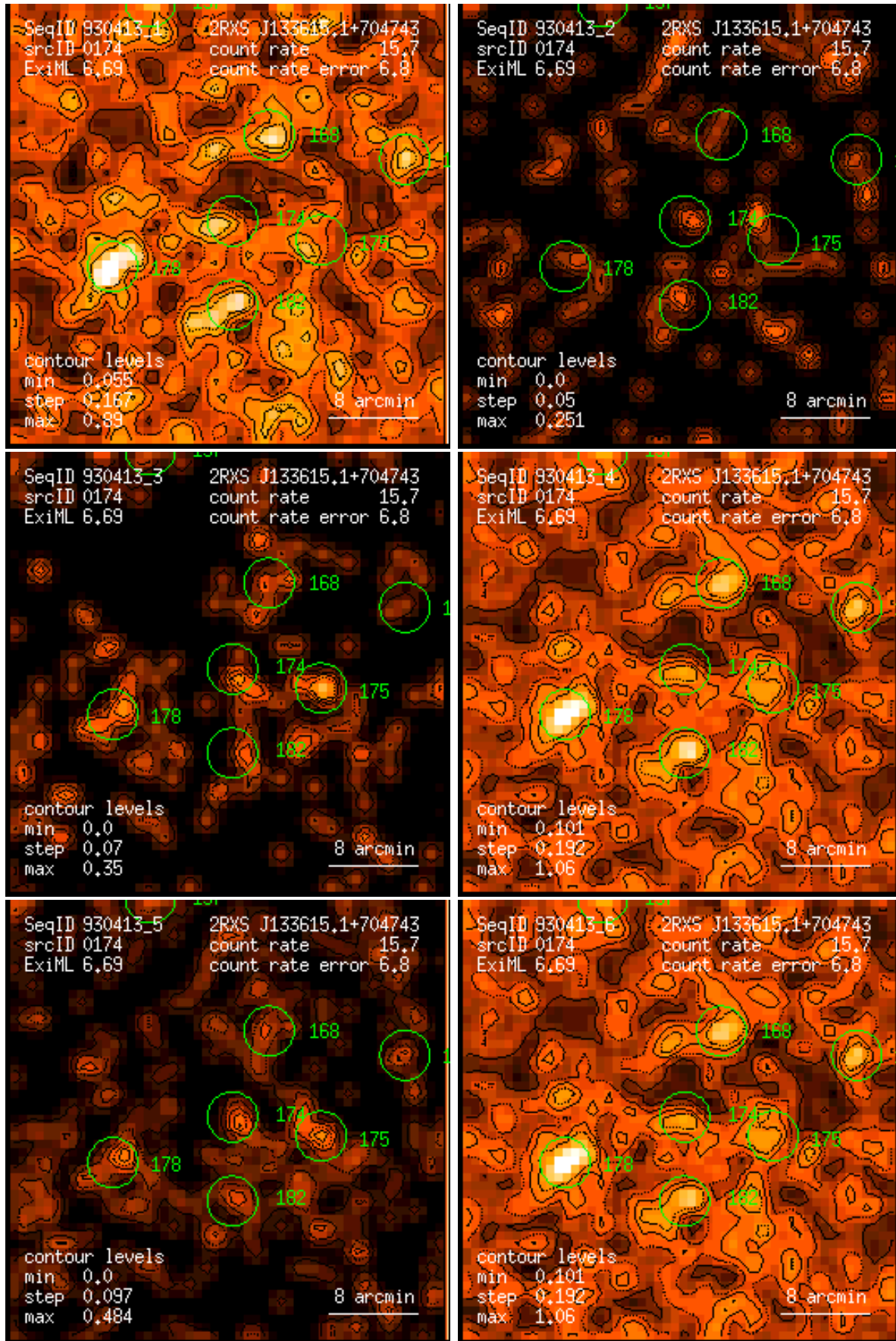
Figure 174: RASS 930413: detection 0174: band rate images, Gaussian filter: (1) PSPC channels 11 – 41, (2) 52 – 90, (3) 91 – 201, (4) 11 – 235, (5) 52 – 201, (6) 11 – 201. Broad band rates in counts/ks. Band rate contour levels in counts/ks/arcmin 2 .
