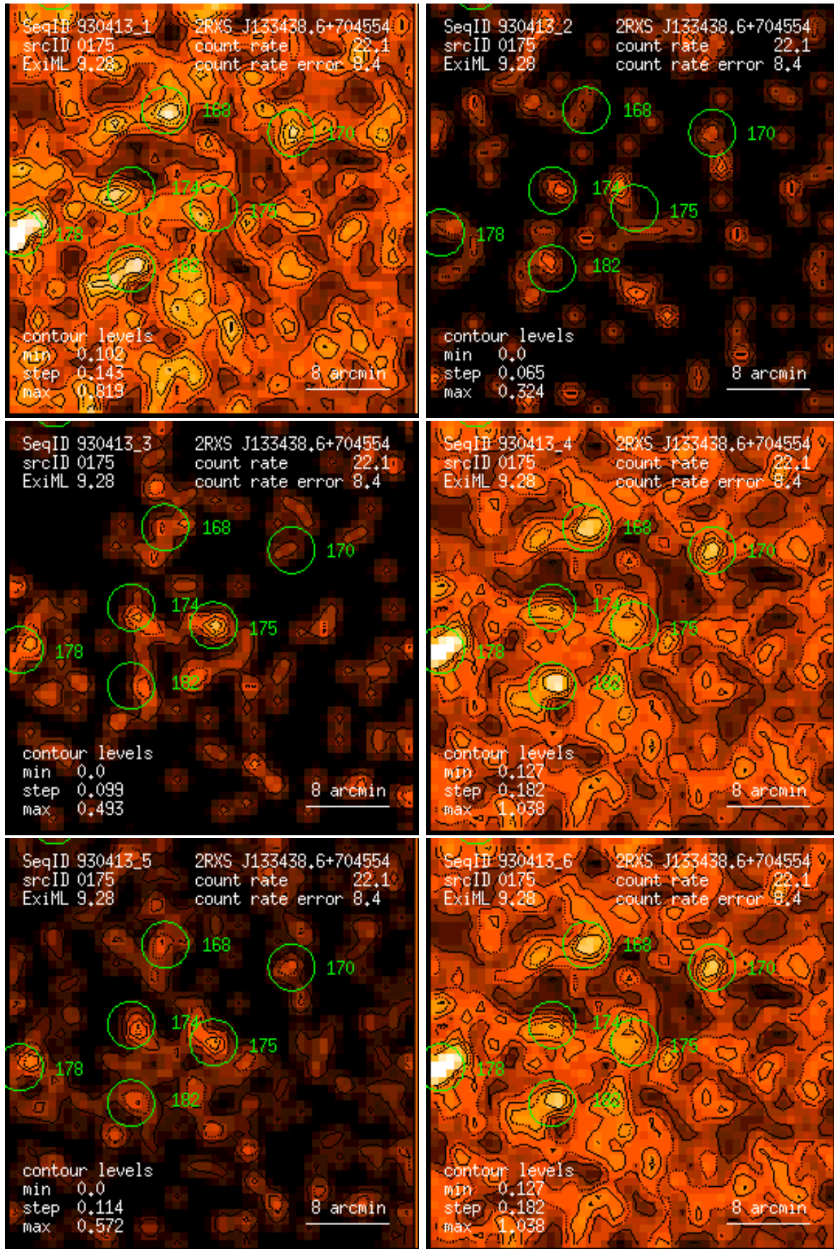
Figure 175: RASS 930413: detection 0175: band rate images, Gaussian filter: (1) PSPC channels 11 – 41, (2) 52 – 90, (3) 91 – 201, (4) 11 – 235, (5) 52 – 201, (6) 11 – 201. Broad band rates in counts/ks. Band rate contour levels in counts/ks/arcmin 2 .
