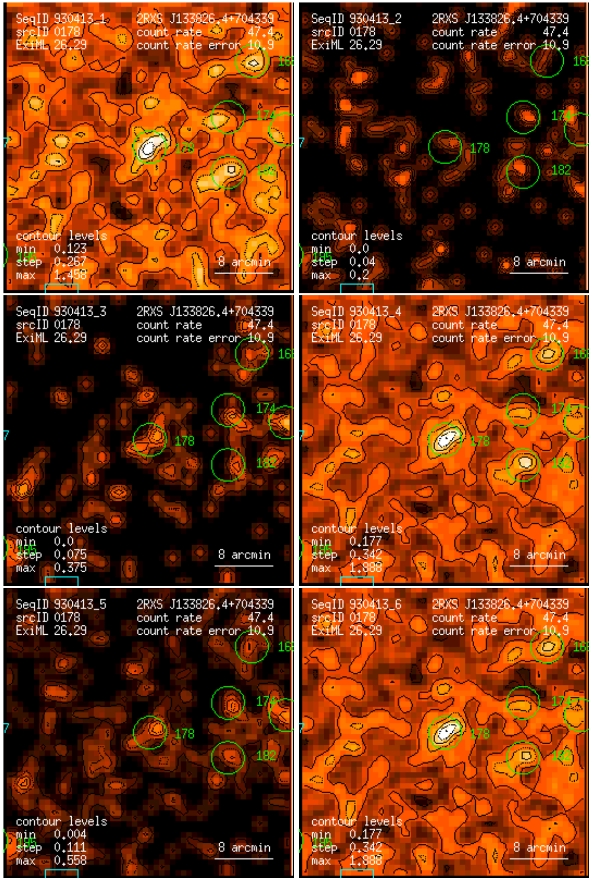
Figure 178: RASS 930413: detection 0178: band rate images, Gaussian filter: (1) PSPC channels 11 – 41, (2) 52 – 90, (3) 91 – 201, (4) 11 – 235, (5) 52 – 201, (6) 11 – 201. Broad band rates in counts/ks. Band rate contour levels in counts/ks/arcmin 2 .
