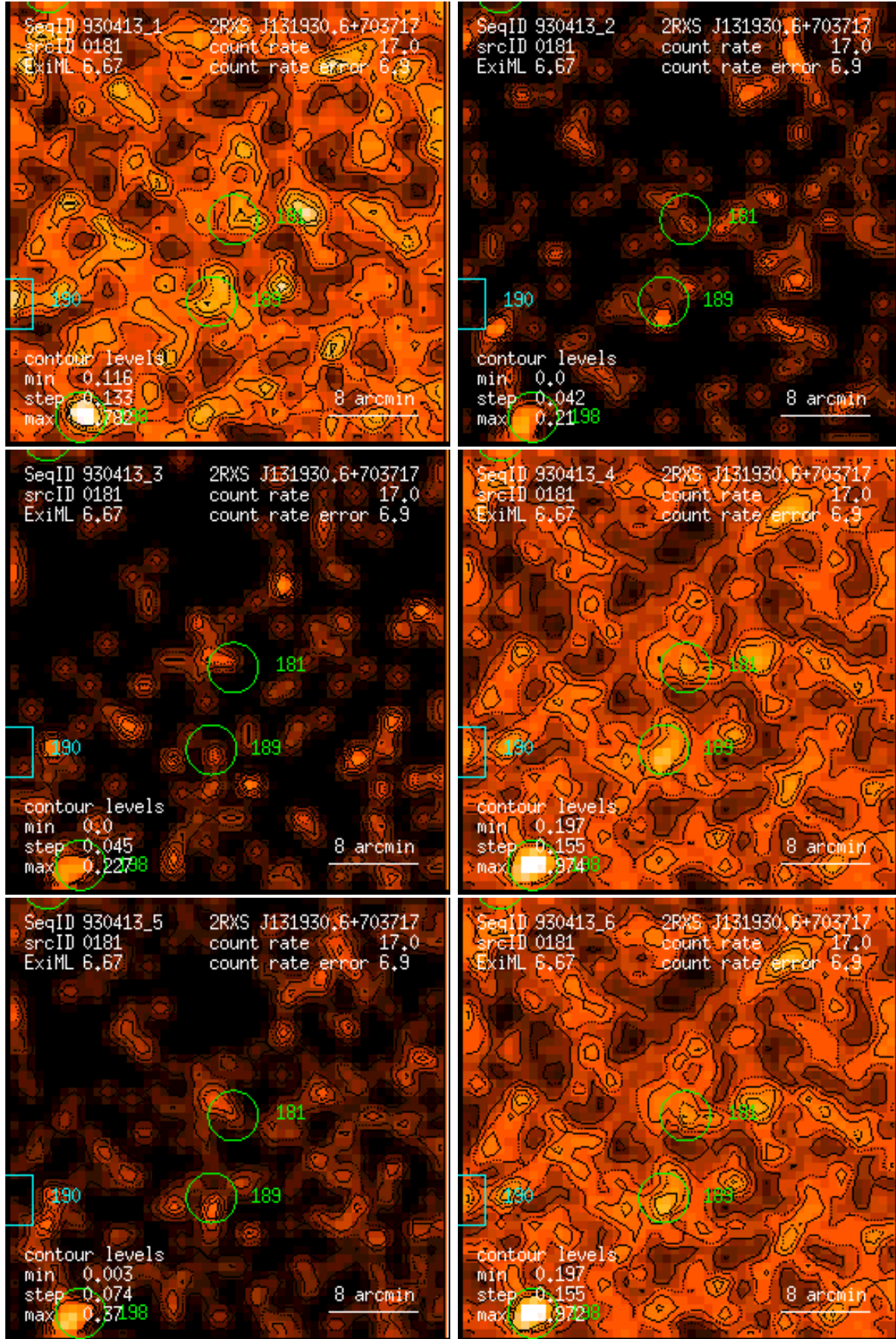
Figure 181: RASS 930413: detection 0181: band rate images, Gaussian filter: (1) PSPC channels 11 – 41, (2) 52 – 90, (3) 91 – 201, (4) 11 – 235, (5) 52 – 201, (6) 11 – 201. Broad band rates in counts/ks. Band rate contour levels in counts/ks/arcmin 2 .
