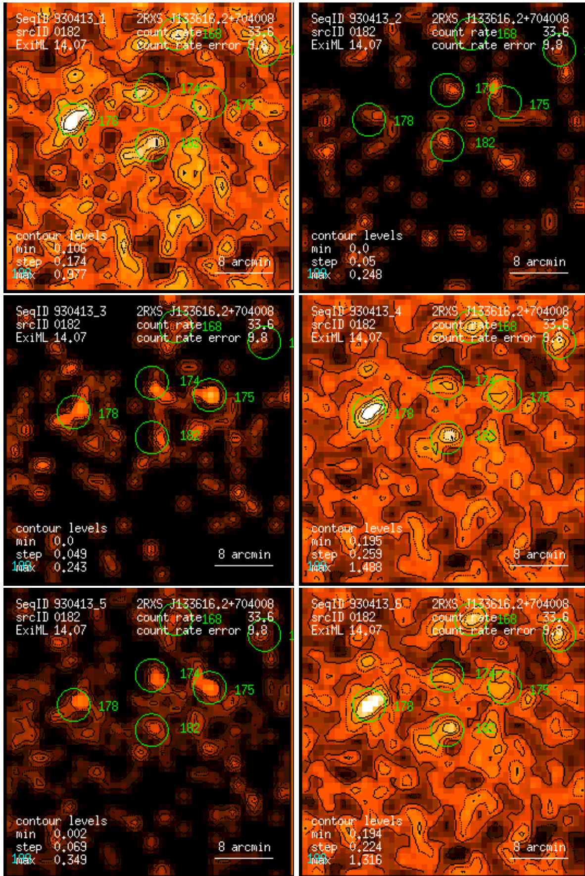
Figure 182: RASS 930413: detection 0182: band rate images, Gaussian filter: (1) PSPC channels 11 – 41, (2) 52 – 90, (3) 91 – 201, (4) 11 – 235, (5) 52 – 201, (6) 11 – 201. Broad band rates in counts/ks. Band rate contour levels in counts/ks/arcmin 2 .
