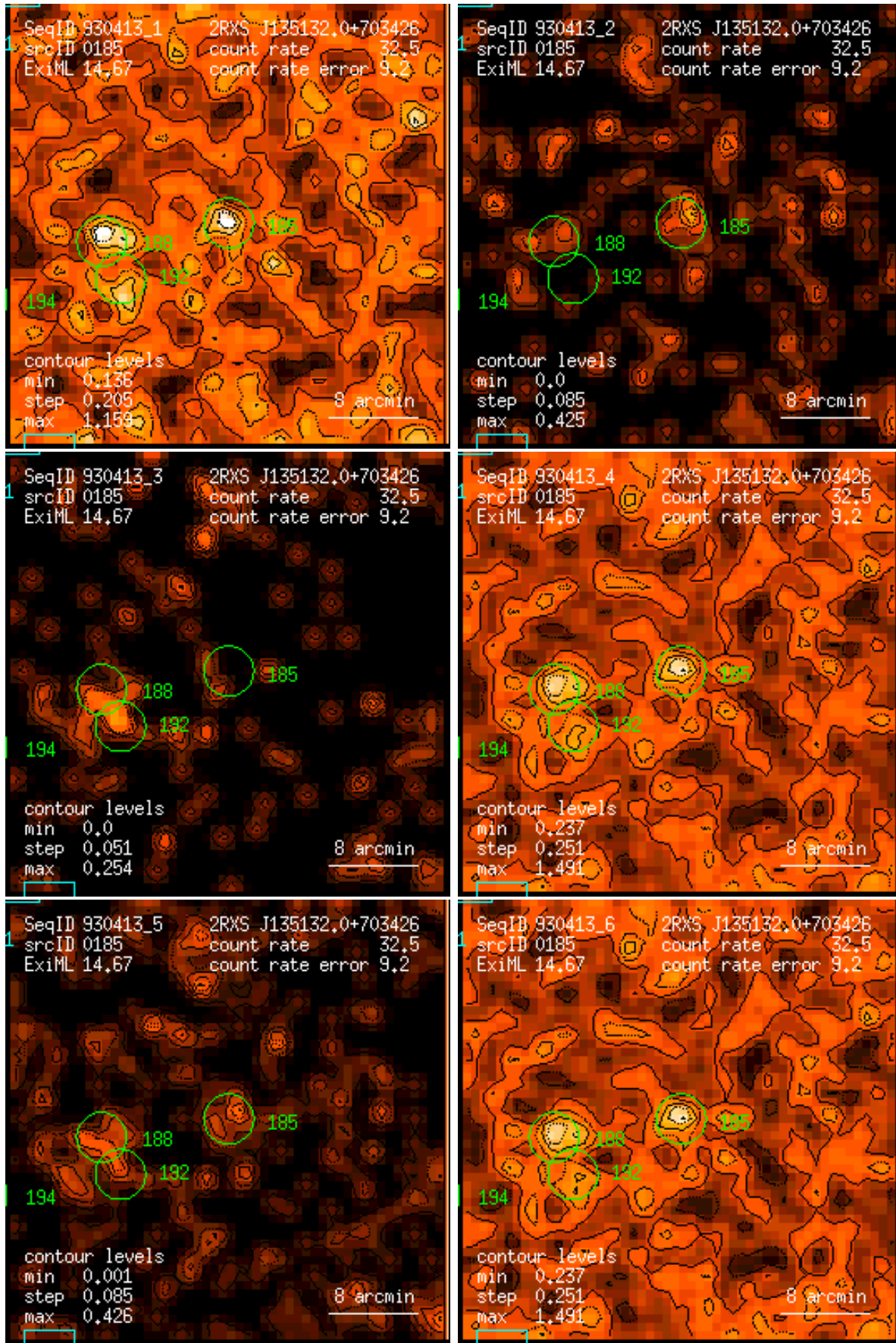
Figure 185: RASS 930413: detection 0185: band rate images, Gaussian filter: (1) PSPC channels 11 – 41, (2) 52 – 90, (3) 91 – 201, (4) 11 – 235, (5) 52 – 201, (6) 11 – 201. Broad band rates in counts/ks. Band rate contour levels in counts/ks/arcmin 2 .
