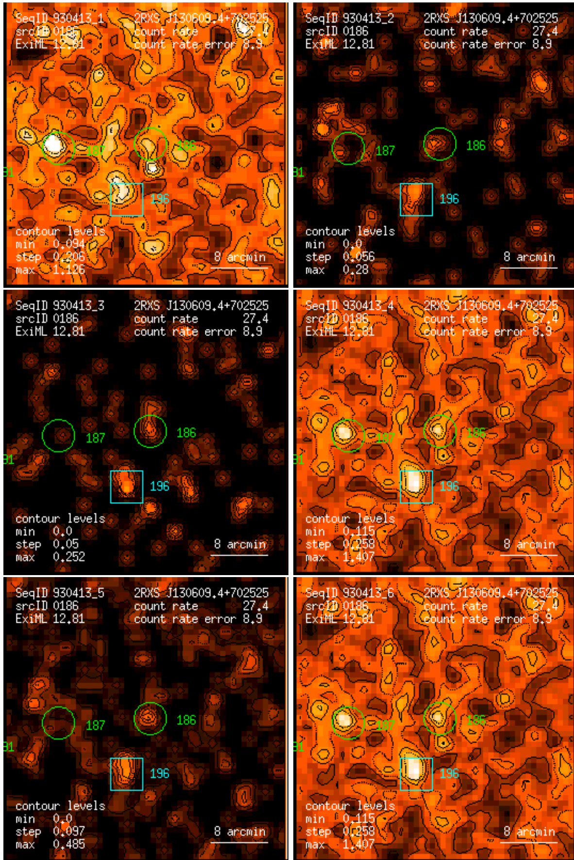
Figure 186: RASS 930413: detection 0186: band rate images, Gaussian filter: (1) PSPC channels 11 – 41, (2) 52 – 90, (3) 91 – 201, (4) 11 – 235, (5) 52 – 201, (6) 11 – 201. Broad band rates in counts/ks. Band rate contour levels in counts/ks/arcmin 2 .
