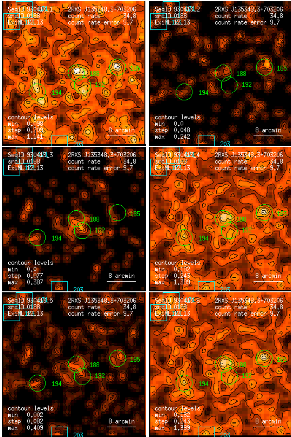
Figure 188: RASS 930413: detection 0188: band rate images, Gaussian filter: (1) PSPC channels 11 – 41, (2) 52 – 90, (3) 91 – 201, (4) 11 – 235, (5) 52 – 201, (6) 11 – 201. Broad band rates in counts/ks. Band rate contour levels in counts/ks/arcmin 2 .
