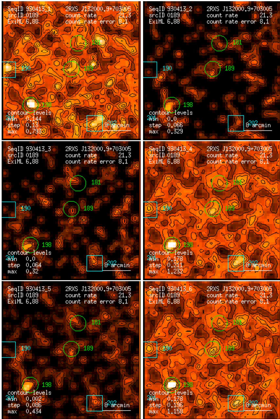
Figure 189: RASS 930413: detection 0189: band rate images, Gaussian filter: (1) PSPC channels 11 – 41, (2) 52 – 90, (3) 91 – 201, (4) 11 – 235, (5) 52 – 201, (6) 11 – 201. Broad band rates in counts/ks. Band rate contour levels in counts/ks/arcmin 2 .
