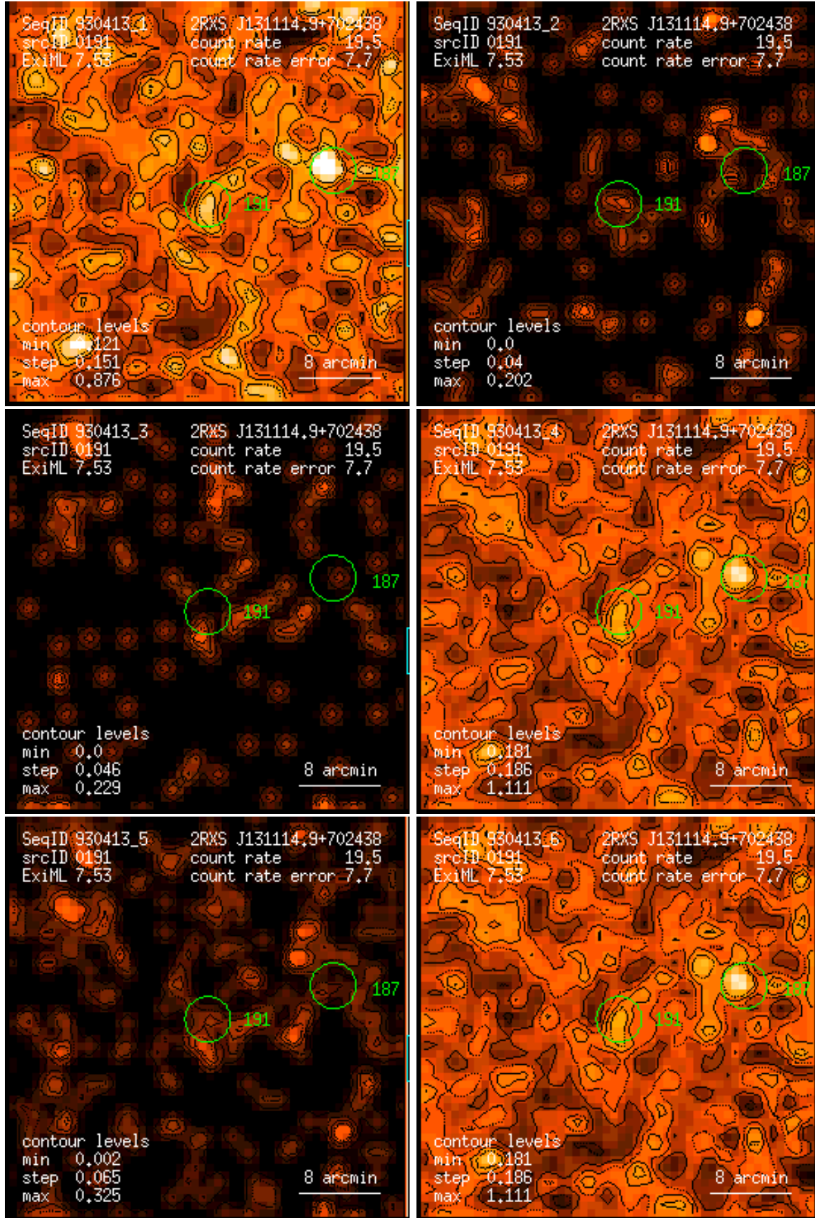
Figure 191: RASS 930413: detection 0191: band rate images, Gaussian filter: (1) PSPC channels 11 – 41, (2) 52 – 90, (3) 91 – 201, (4) 11 – 235, (5) 52 – 201, (6) 11 – 201. Broad band rates in counts/ks. Band rate contour levels in counts/ks/arcmin 2 .
