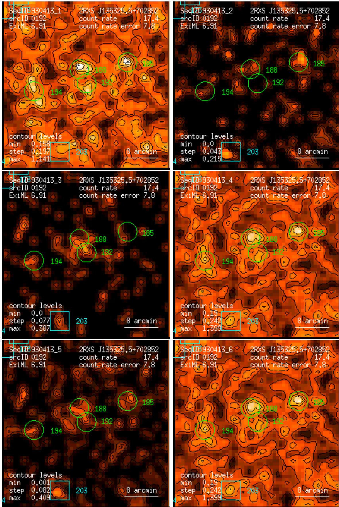
Figure 192: RASS 930413: detection 0192: band rate images, Gaussian filter: (1) PSPC channels 11 – 41, (2) 52 – 90, (3) 91 – 201, (4) 11 – 235, (5) 52 – 201, (6) 11 – 201. Broad band rates in counts/ks. Band rate contour levels in counts/ks/arcmin 2 .
