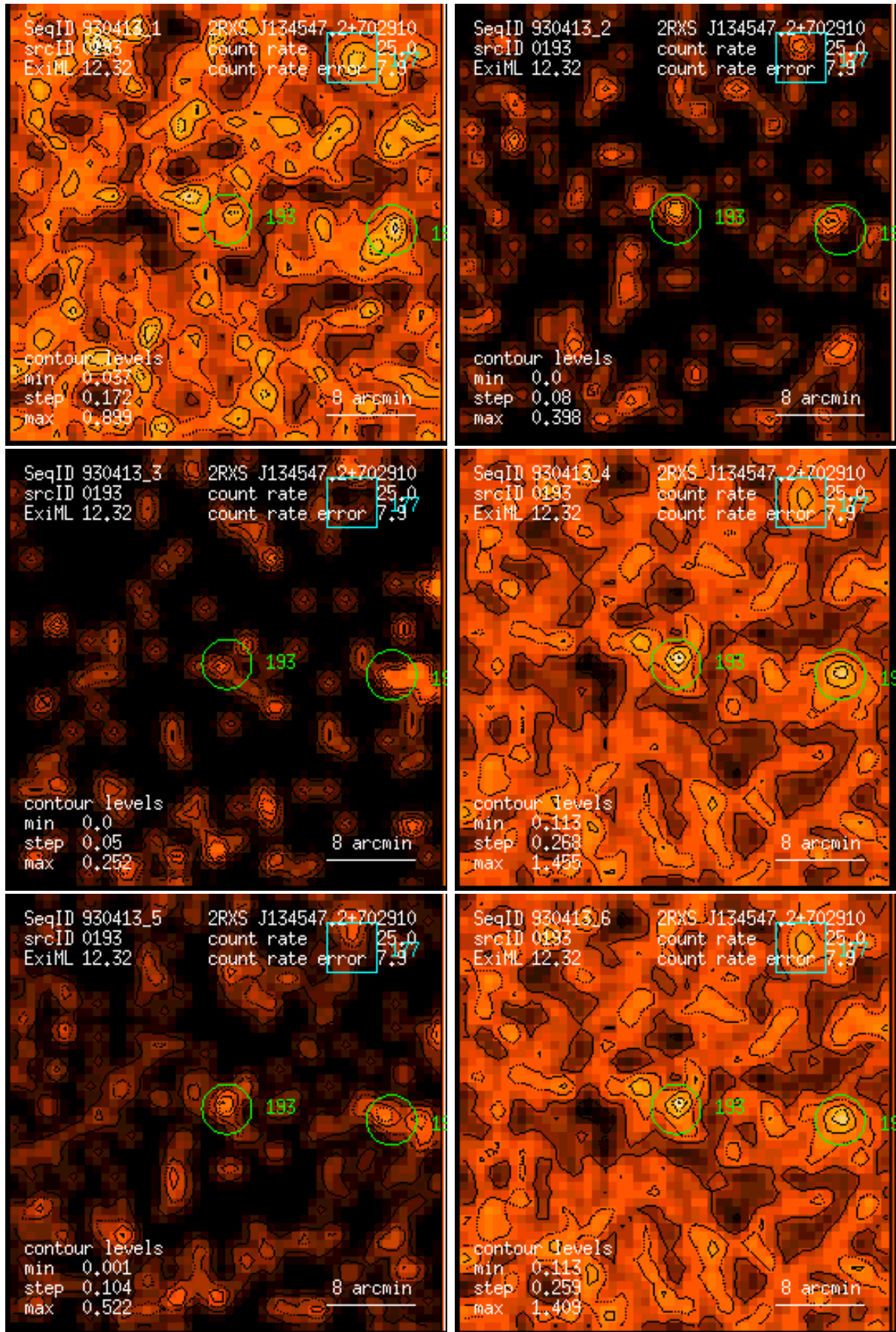
Figure 193: RASS 930413: detection 0193: band rate images, Gaussian filter: (1) PSPC channels 11 – 41, (2) 52 – 90, (3) 91 – 201, (4) 11 – 235, (5) 52 – 201, (6) 11 – 201. Broad band rates in counts/ks. Band rate contour levels in counts/ks/arcmin 2 .
