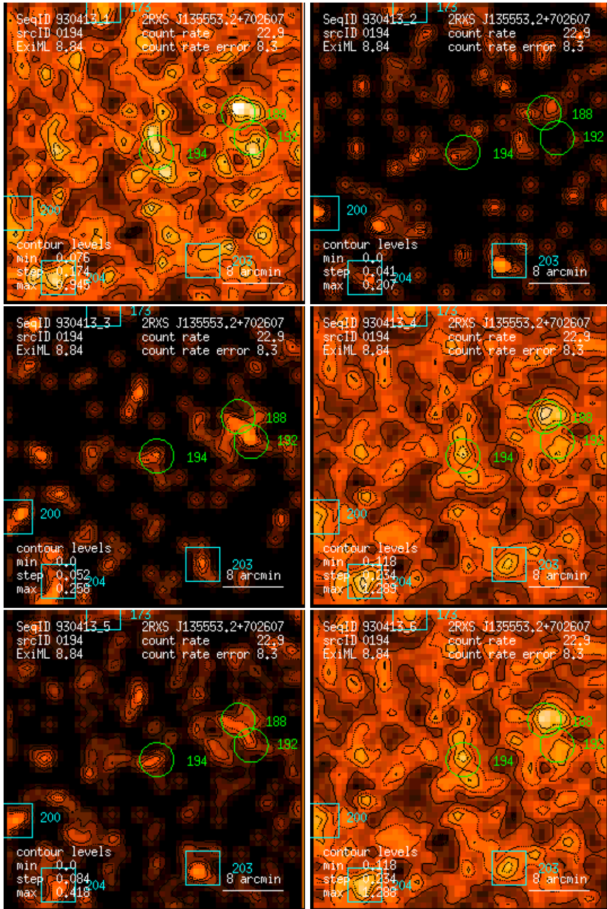
Figure 194: RASS 930413: detection 0194: band rate images, Gaussian filter: (1) PSPC channels 11 – 41, (2) 52 – 90, (3) 91 – 201, (4) 11 – 235, (5) 52 – 201, (6) 11 – 201. Broad band rates in counts/ks. Band rate contour levels in counts/ks/arcmin 2 .
