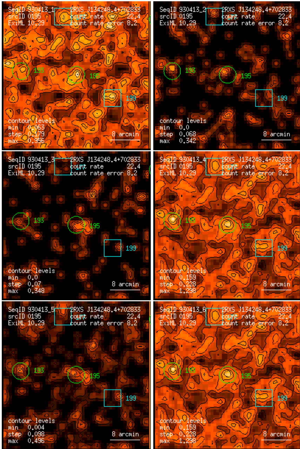
Figure 195: RASS 930413: detection 0195: band rate images, Gaussian filter: (1) PSPC channels 11 – 41, (2) 52 – 90, (3) 91 – 201, (4) 11 – 235, (5) 52 – 201, (6) 11 – 201. Broad band rates in counts/ks. Band rate contour levels in counts/ks/arcmin 2 .
