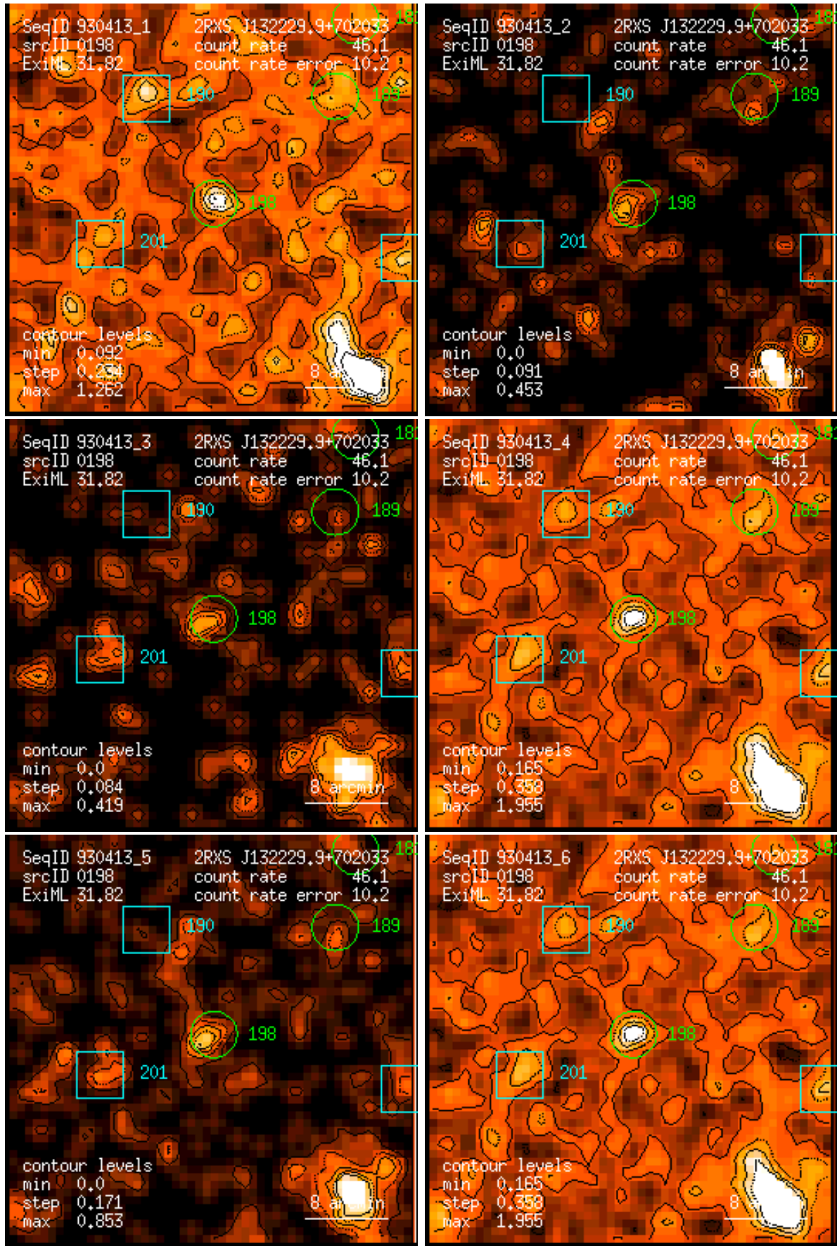
Figure 198: RASS 930413: detection 0198: band rate images, Gaussian filter: (1) PSPC channels 11 – 41, (2) 52 – 90, (3) 91 – 201, (4) 11 – 235, (5) 52 – 201, (6) 11 – 201. Broad band rates in counts/ks. Band rate contour levels in counts/ks/arcmin 2 .
