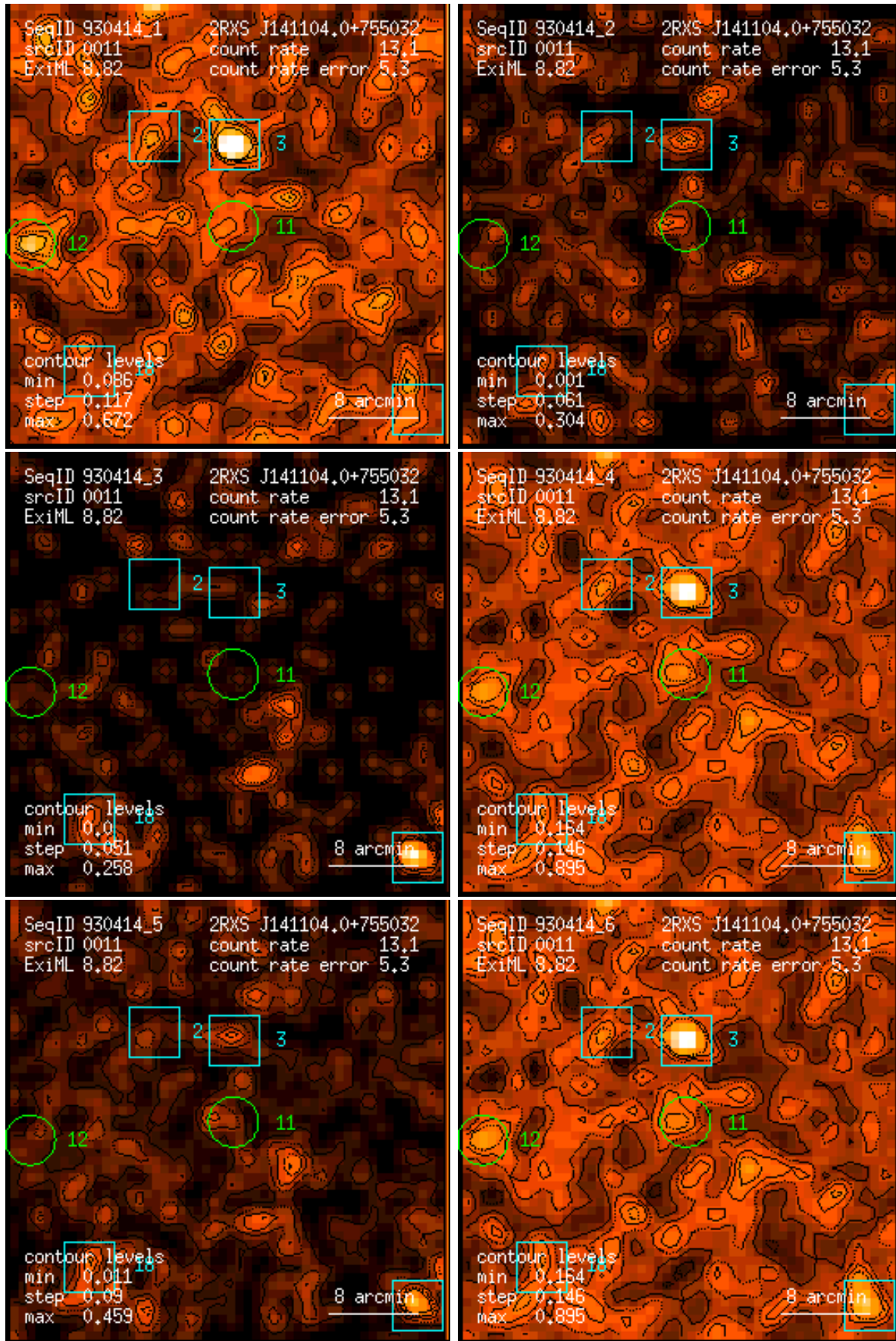
Figure 11: RASS 930414: detection 0011: band rate images, Gaussian filter: (1) PSPC channels 11 – 41, (2) 52 – 90, (3) 91 – 201, (4) 11 – 235, (5) 52 – 201, (6) 11 – 201. Broad band rates in counts/ks. Band rate contour levels in counts/ks/arcmin 2 .
