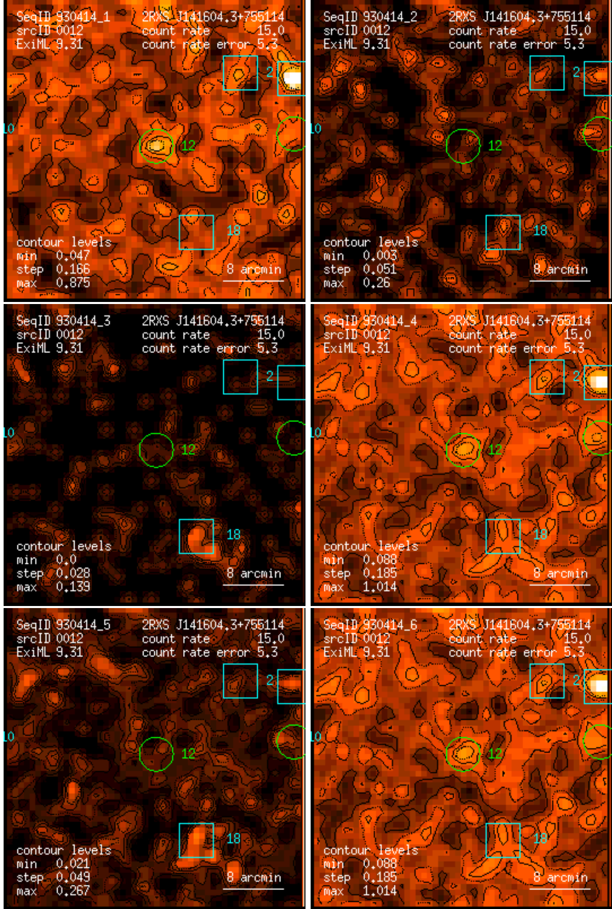
Figure 12: RASS 930414: detection 0012: band rate images, Gaussian filter: (1) PSPC channels 11 – 41, (2) 52 – 90, (3) 91 – 201, (4) 11 – 235, (5) 52 – 201, (6) 11 – 201. Broad band rates in counts/ks. Band rate contour levels in counts/ks/arcmin 2 .
