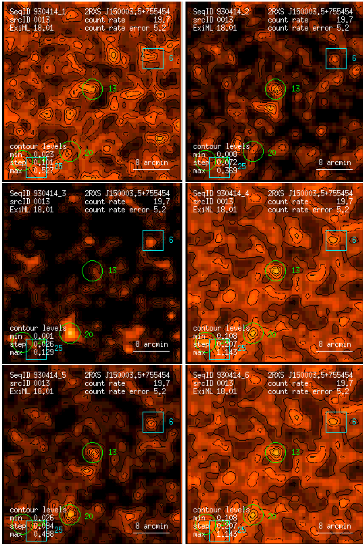
Figure 13: RASS 930414: detection 0013: band rate images, Gaussian filter: (1) PSPC channels 11 – 41, (2) 52 – 90, (3) 91 – 201, (4) 11 – 235, (5) 52 – 201, (6) 11 – 201. Broad band rates in counts/ks. Band rate contour levels in counts/ks/arcmin 2 .
