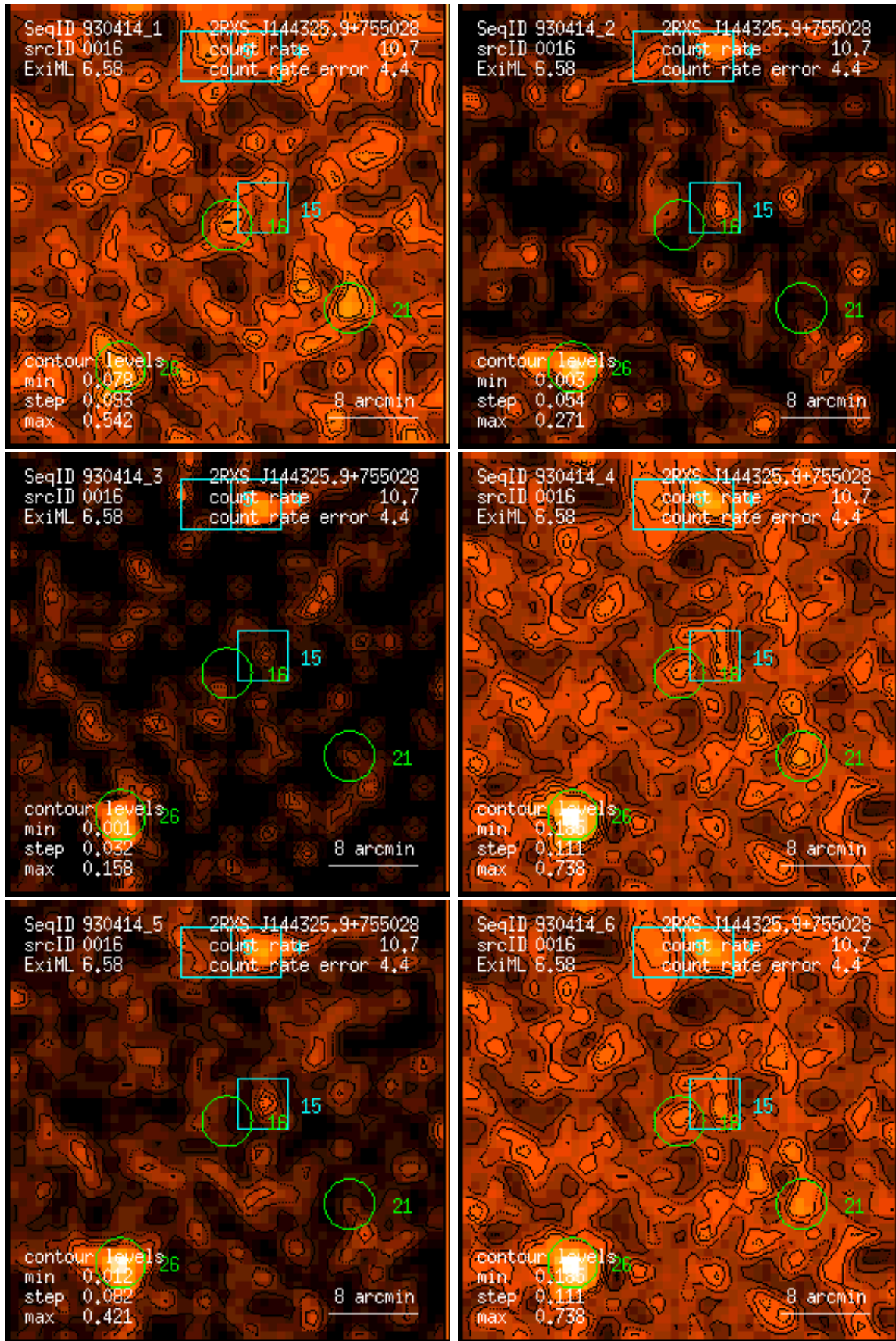
Figure 16: RASS 930414: detection 0016: band rate images, Gaussian filter: (1) PSPC channels 11 – 41, (2) 52 – 90, (3) 91 – 201, (4) 11 – 235, (5) 52 – 201, (6) 11 – 201. Broad band rates in counts/ks. Band rate contour levels in counts/ks/arcmin 2 .
