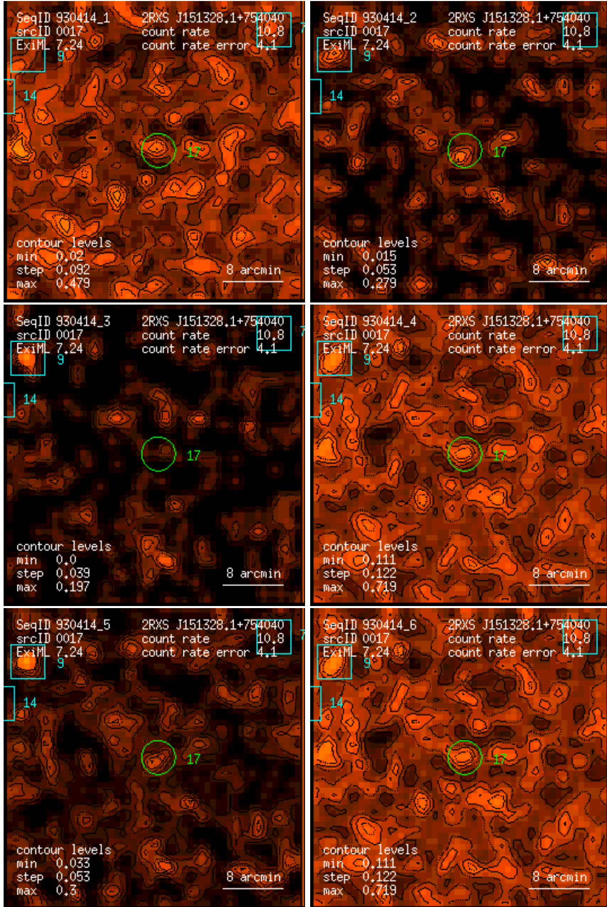
Figure 17: RASS 930414: detection 0017: band rate images, Gaussian filter: (1) PSPC channels 11 – 41, (2) 52 – 90, (3) 91 – 201, (4) 11 – 235, (5) 52 – 201, (6) 11 – 201. Broad band rates in counts/ks. Band rate contour levels in counts/ks/arcmin 2 .
