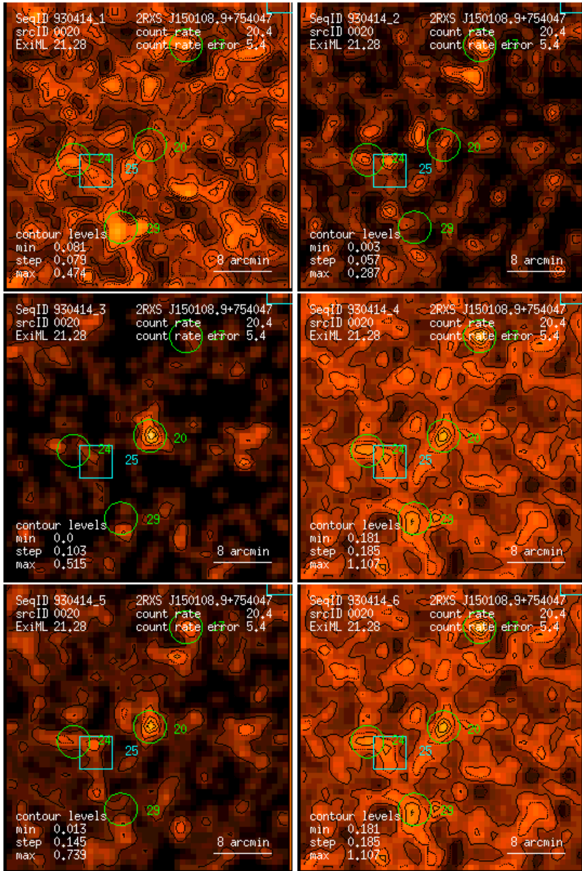
Figure 20: RASS 930414: detection 0020: band rate images, Gaussian filter: (1) PSPC channels 11 – 41, (2) 52 – 90, (3) 91 – 201, (4) 11 – 235, (5) 52 – 201, (6) 11 – 201. Broad band rates in counts/ks. Band rate contour levels in counts/ks/arcmin 2 .
