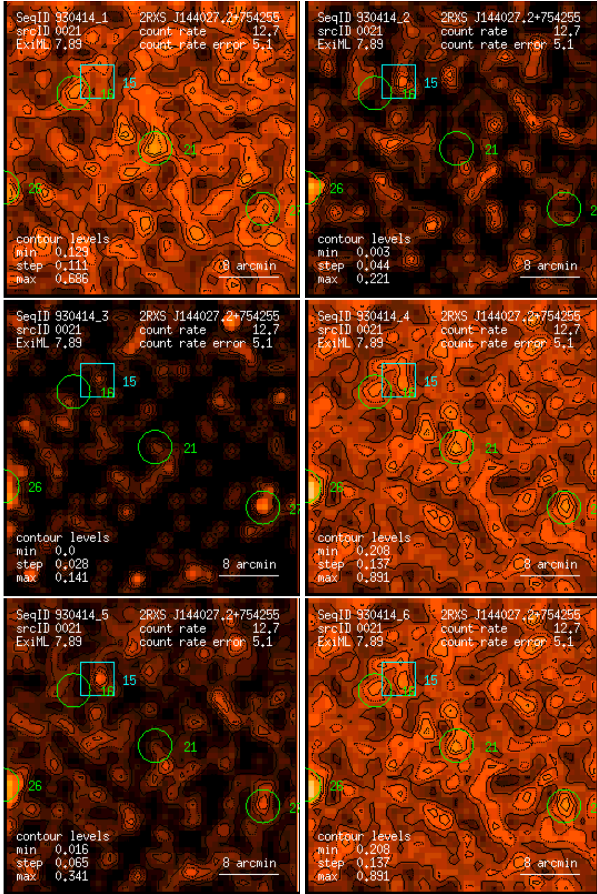
Figure 21: RASS 930414: detection 0021: band rate images, Gaussian filter: (1) PSPC channels 11 – 41, (2) 52 – 90, (3) 91 – 201, (4) 11 – 235, (5) 52 – 201, (6) 11 – 201. Broad band rates in counts/ks. Band rate contour levels in counts/ks/arcmin 2 .
