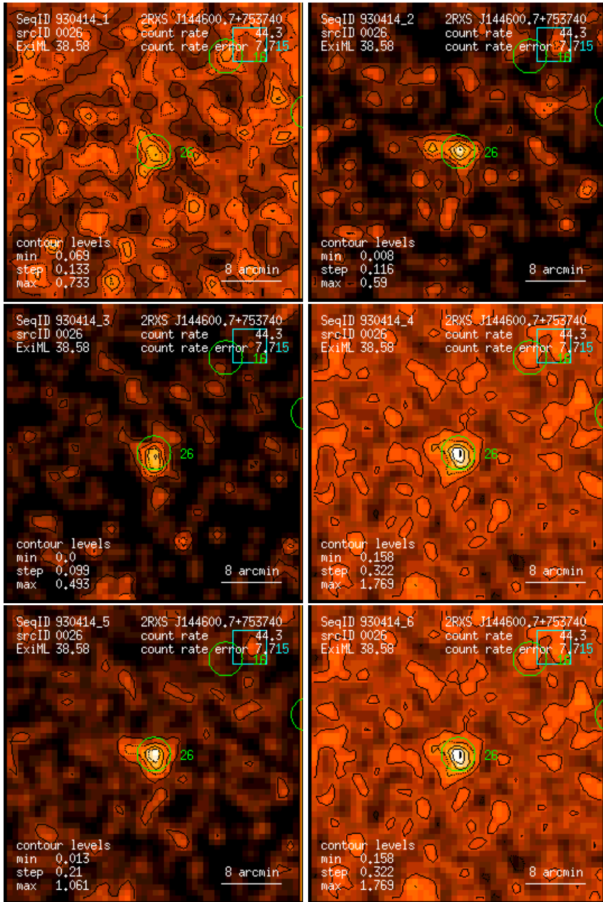
Figure 26: RASS 930414: detection 0026: band rate images, Gaussian filter: (1) PSPC channels 11 – 41, (2) 52 – 90, (3) 91 – 201, (4) 11 – 235, (5) 52 – 201, (6) 11 – 201. Broad band rates in counts/ks. Band rate contour levels in counts/ks/arcmin 2 .
