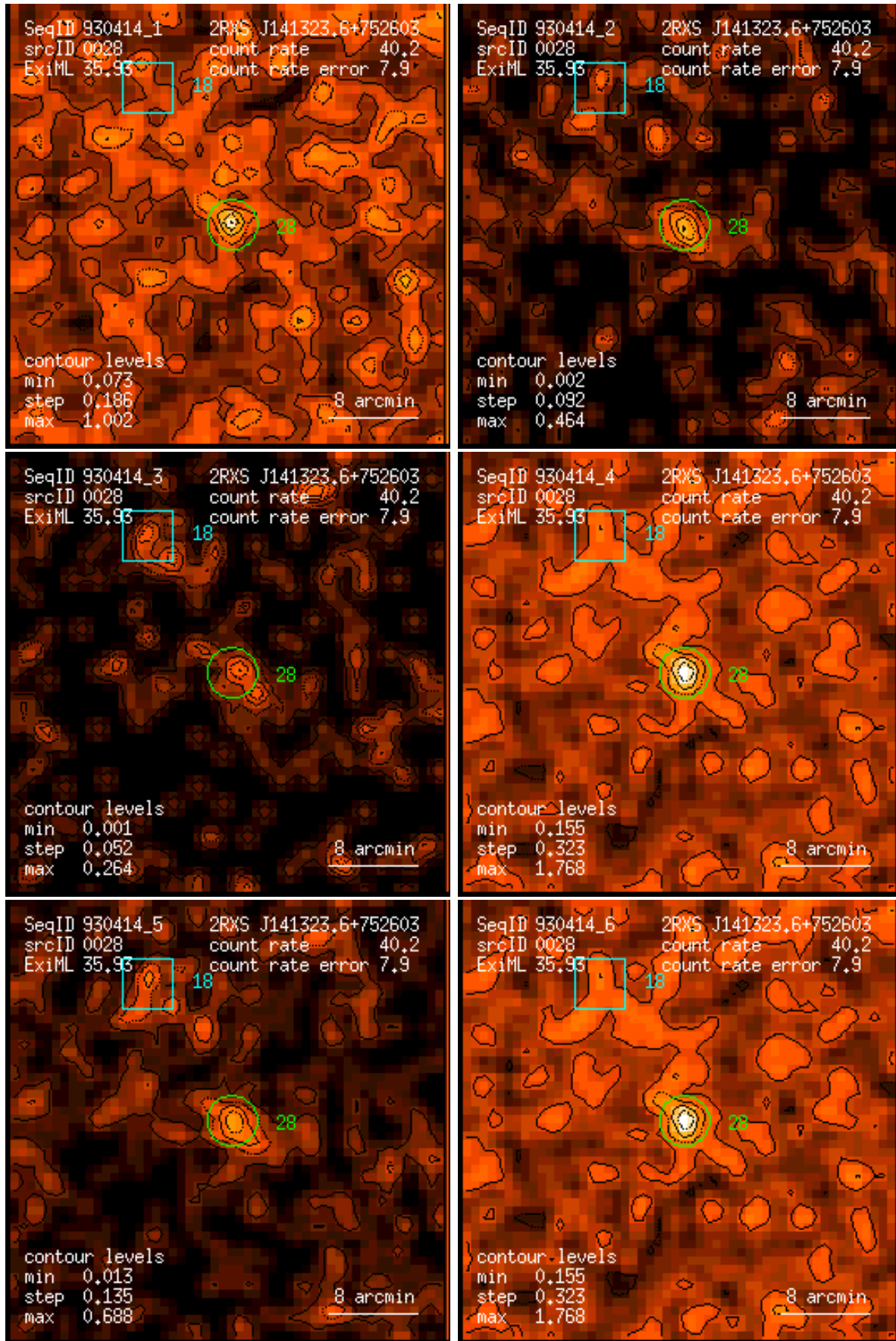
Figure 28: RASS 930414: detection 0028: band rate images, Gaussian filter: (1) PSPC channels 11 – 41, (2) 52 – 90, (3) 91 – 201, (4) 11 – 235, (5) 52 – 201, (6) 11 – 201. Broad band rates in counts/ks. Band rate contour levels in counts/ks/arcmin 2 .
