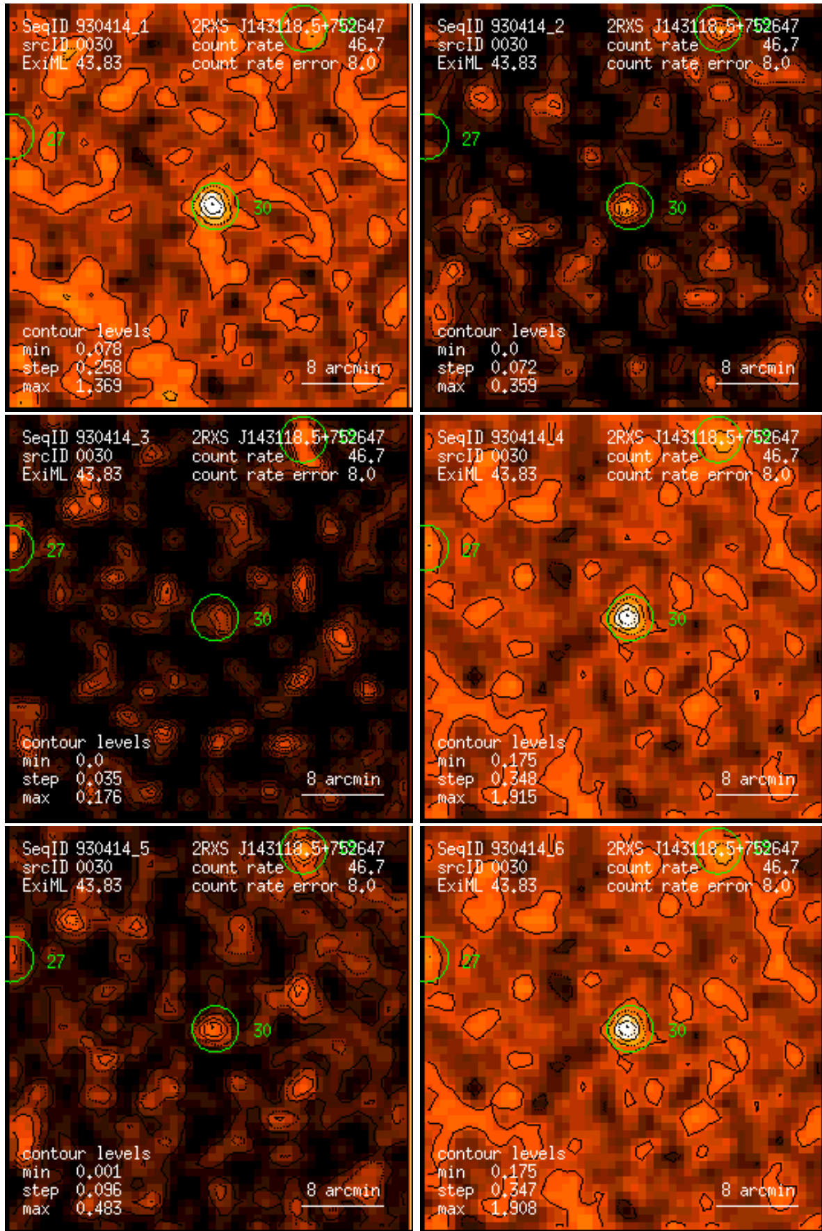
Figure 30: RASS 930414: detection 0030: band rate images, Gaussian filter: (1) PSPC channels 11 – 41, (2) 52 – 90, (3) 91 – 201, (4) 11 – 235, (5) 52 – 201, (6) 11 – 201. Broad band rates in counts/ks. Band rate contour levels in counts/ks/arcmin 2 .
