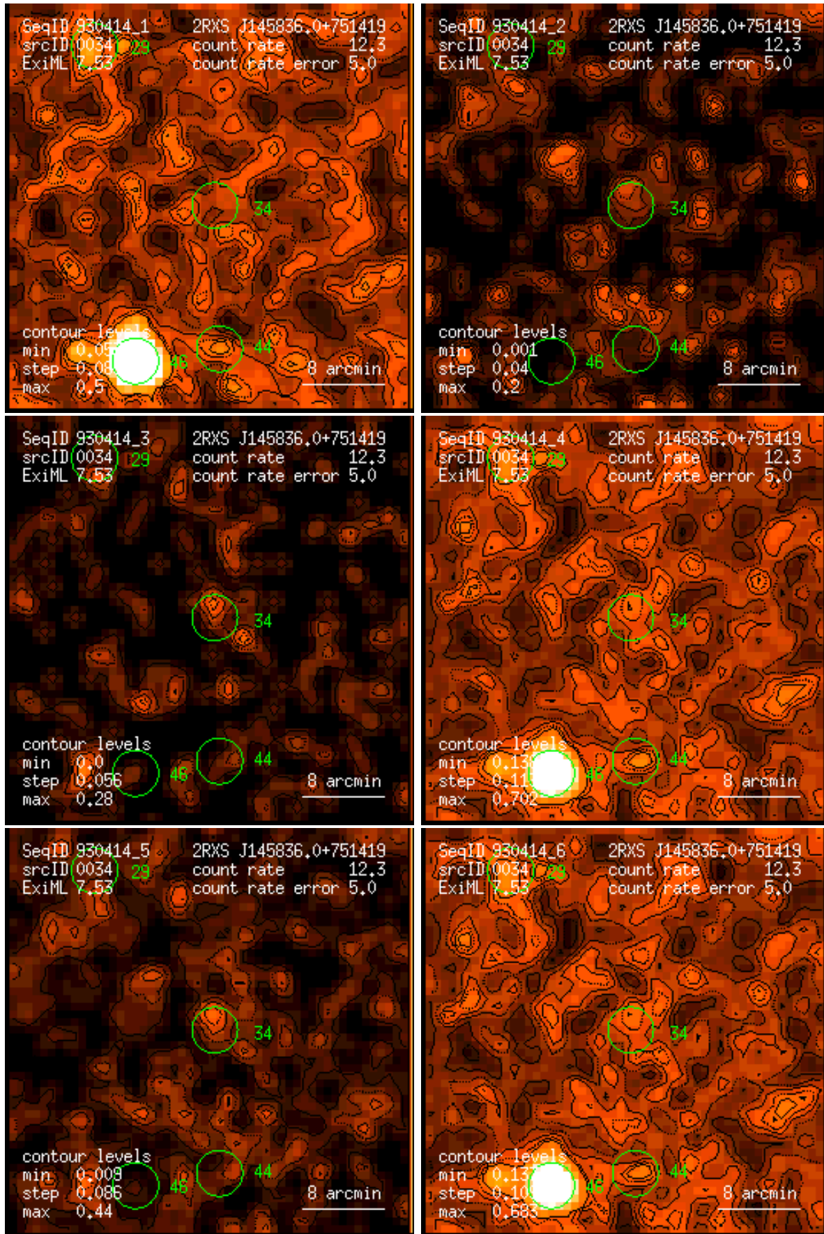
Figure 34: RASS 930414: detection 0034: band rate images, Gaussian filter: (1) PSPC channels 11 – 41, (2) 52 – 90, (3) 91 – 201, (4) 11 – 235, (5) 52 – 201, (6) 11 – 201. Broad band rates in counts/ks. Band rate contour levels in counts/ks/arcmin 2 .
