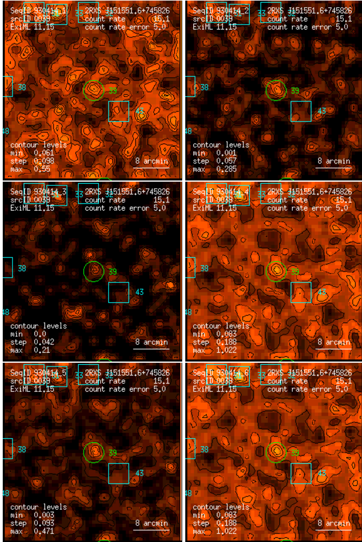
Figure 39: RASS 930414: detection 0039: band rate images, Gaussian filter: (1) PSPC channels 11 – 41, (2) 52 – 90, (3) 91 – 201, (4) 11 – 235, (5) 52 – 201, (6) 11 – 201. Broad band rates in counts/ks. Band rate contour levels in counts/ks/arcmin 2 .
