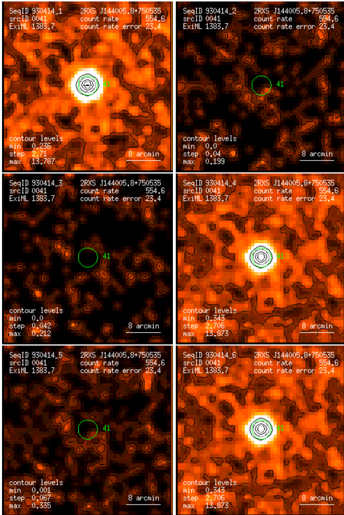
Figure 41: RASS 930414: detection 0041: band rate images, Gaussian filter: (1) PSPC channels 11 – 41, (2) 52 – 90, (3) 91 – 201, (4) 11 – 235, (5) 52 – 201, (6) 11 – 201. Broad band rates in counts/ks. Band rate contour levels in counts/ks/arcmin 2 .
