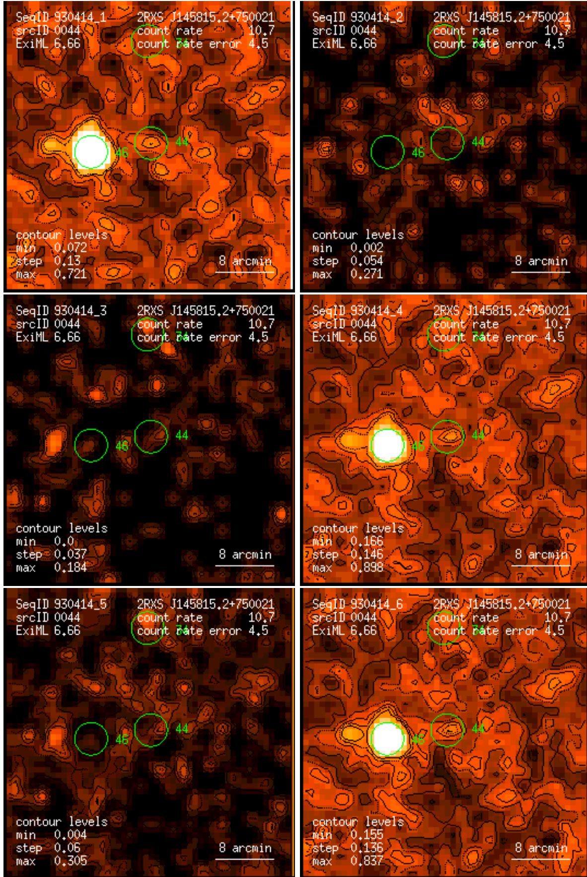
Figure 44: RASS 930414: detection 0044: band rate images, Gaussian filter: (1) PSPC channels 11 – 41, (2) 52 – 90, (3) 91 – 201, (4) 11 – 235, (5) 52 – 201, (6) 11 – 201. Broad band rates in counts/ks. Band rate contour levels in counts/ks/arcmin 2 .
