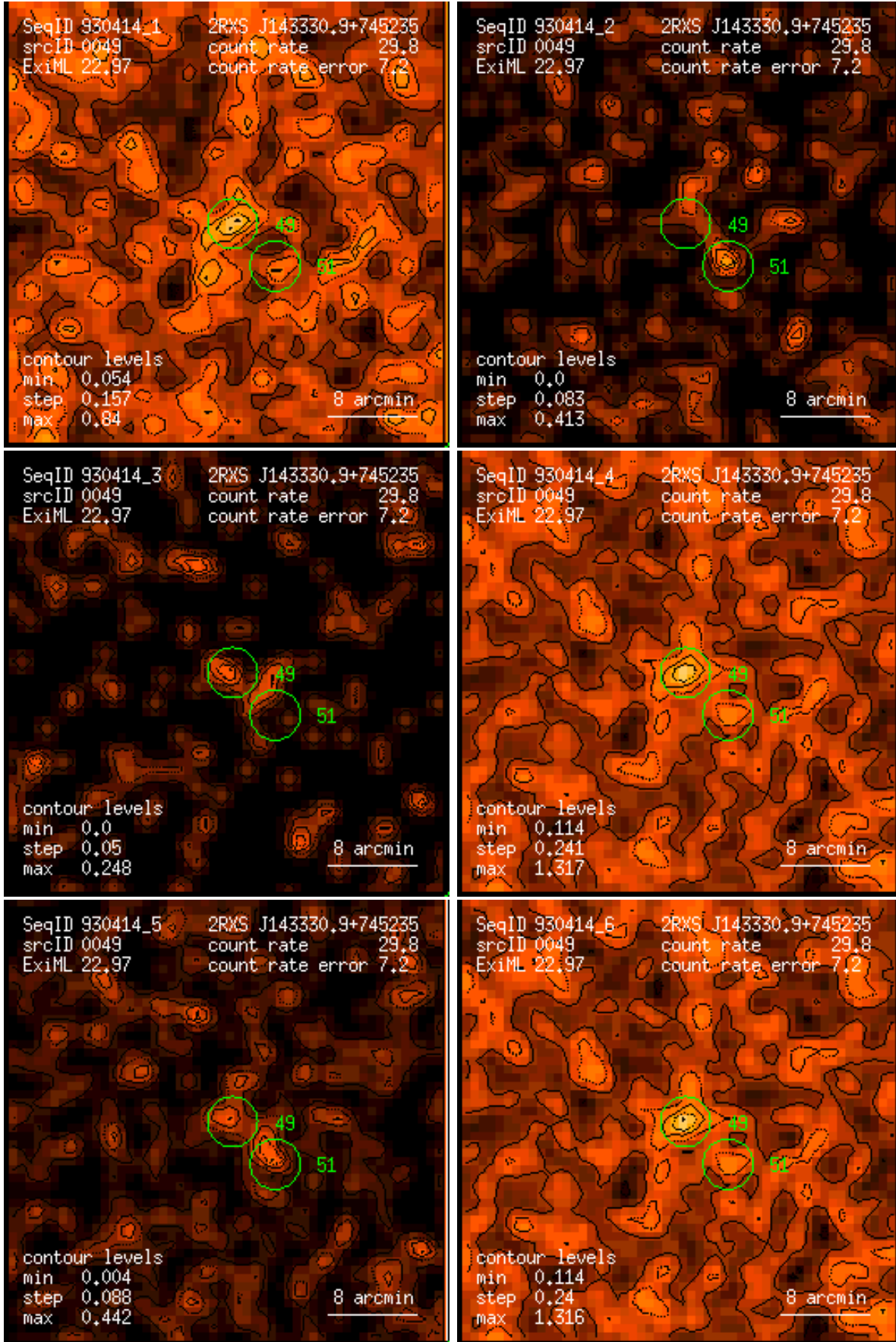
Figure 49: RASS 930414: detection 0049: band rate images, Gaussian filter: (1) PSPC channels 11 – 41, (2) 52 – 90, (3) 91 – 201, (4) 11 – 235, (5) 52 – 201, (6) 11 – 201. Broad band rates in counts/ks. Band rate contour levels in counts/ks/arcmin 2 .
