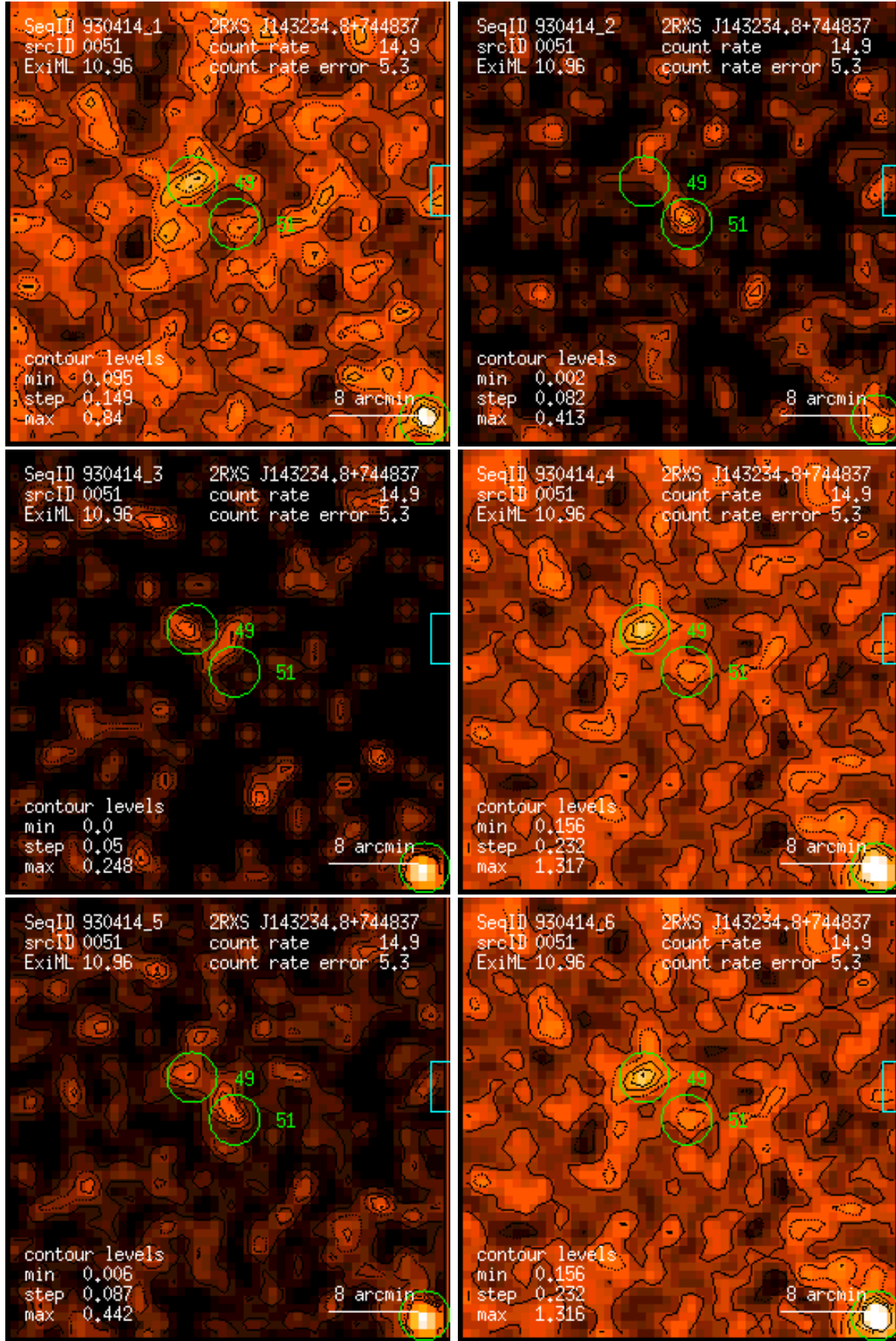
Figure 51: RASS 930414: detection 0051: band rate images, Gaussian filter: (1) PSPC channels 11 – 41, (2) 52 – 90, (3) 91 – 201, (4) 11 – 235, (5) 52 – 201, (6) 11 – 201. Broad band rates in counts/ks. Band rate contour levels in counts/ks/arcmin 2 .
