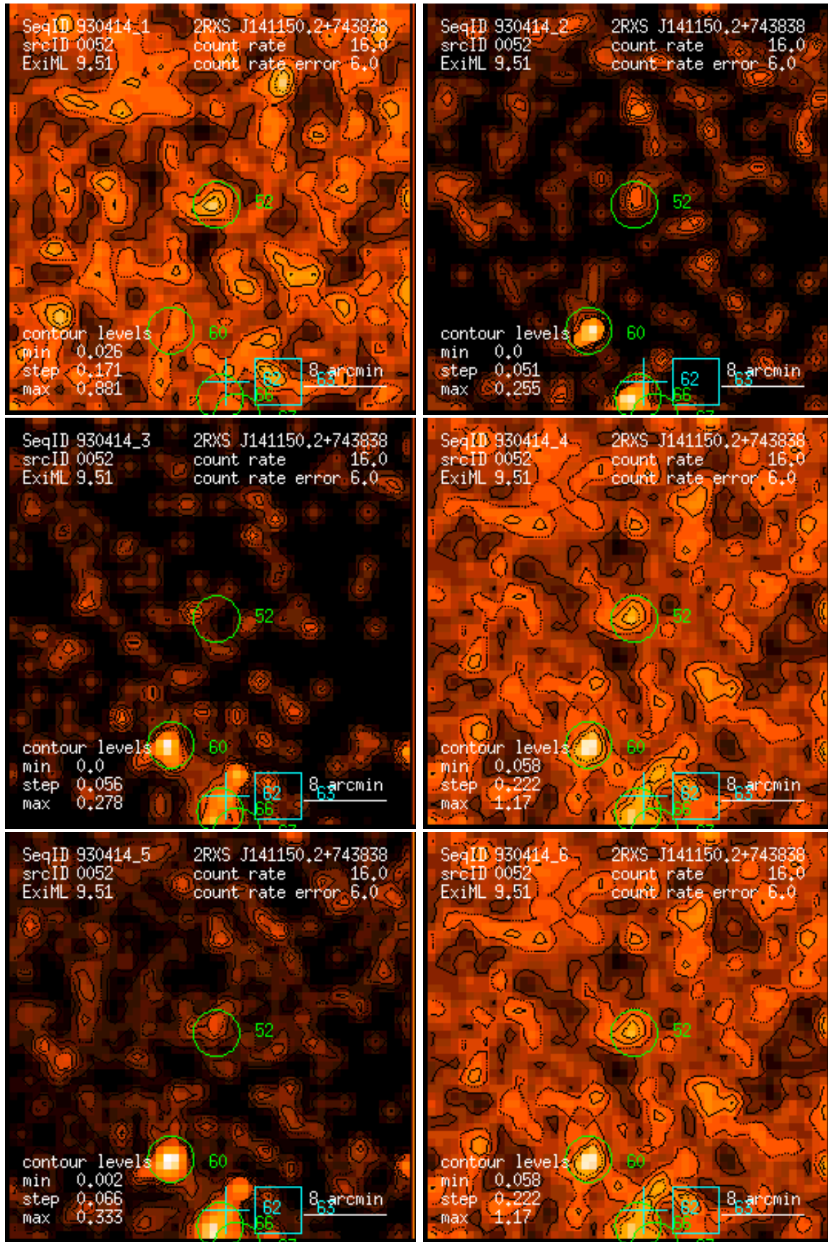
Figure 52: RASS 930414: detection 0052: band rate images, Gaussian filter: (1) PSPC channels 11 – 41, (2) 52 – 90, (3) 91 – 201, (4) 11 – 235, (5) 52 – 201, (6) 11 – 201. Broad band rates in counts/ks. Band rate contour levels in counts/ks/arcmin 2 .
