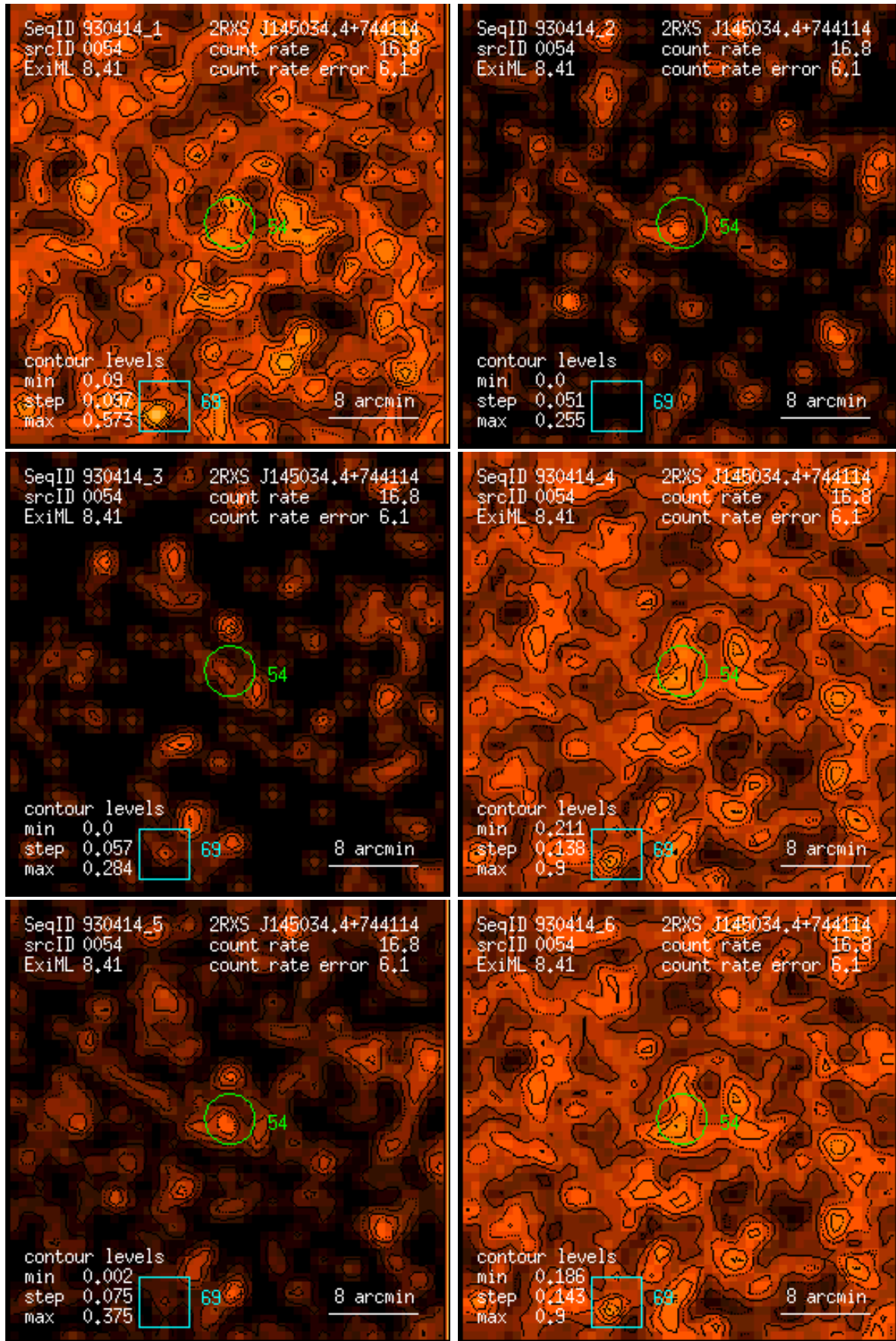
Figure 54: RASS 930414: detection 0054: band rate images, Gaussian filter: (1) PSPC channels 11 – 41, (2) 52 – 90, (3) 91 – 201, (4) 11 – 235, (5) 52 – 201, (6) 11 – 201. Broad band rates in counts/ks. Band rate contour levels in counts/ks/arcmin 2 .
