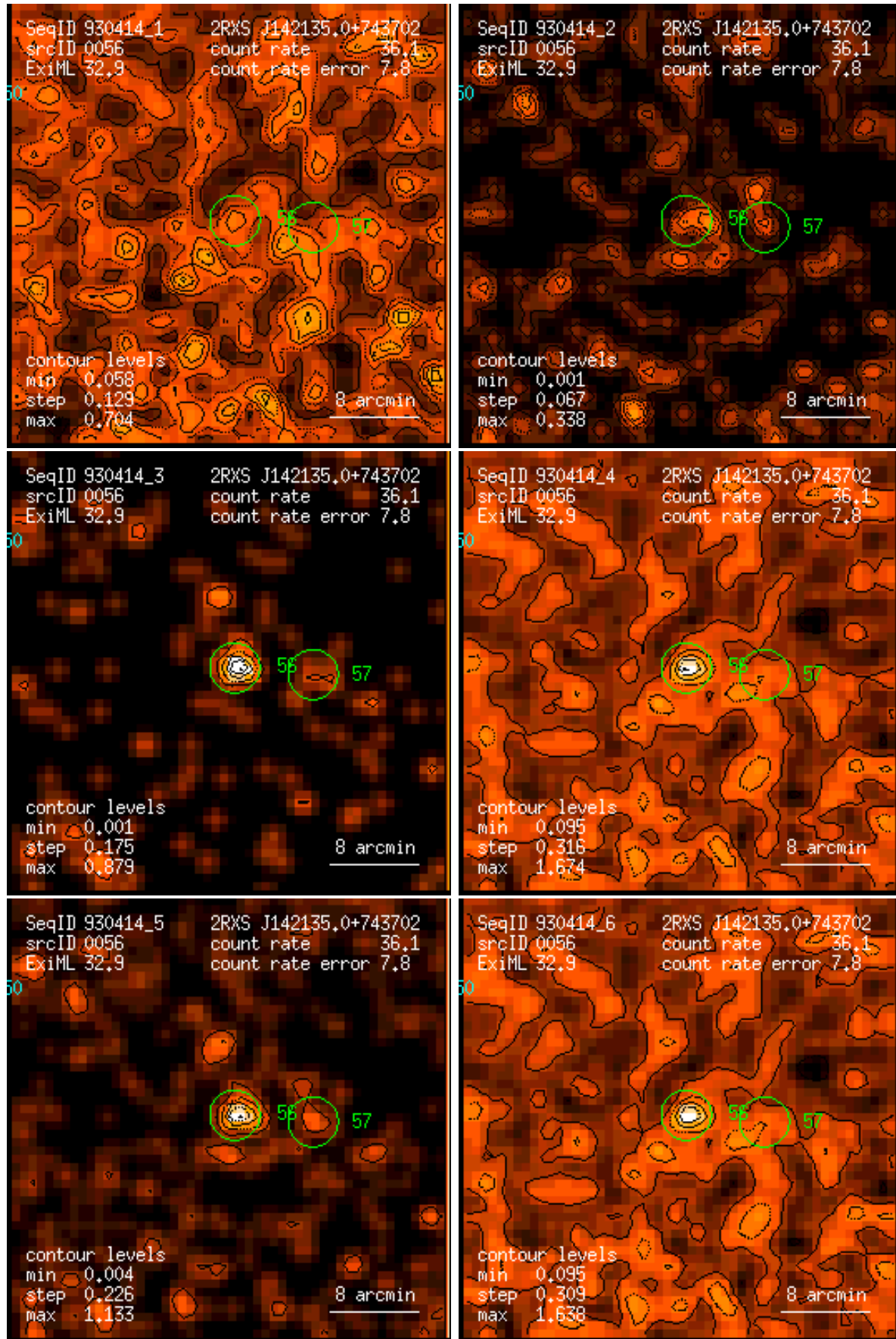
Figure 56: RASS 930414: detection 0056: band rate images, Gaussian filter: (1) PSPC channels 11 – 41, (2) 52 – 90, (3) 91 – 201, (4) 11 – 235, (5) 52 – 201, (6) 11 – 201. Broad band rates in counts/ks. Band rate contour levels in counts/ks/arcmin 2 .
