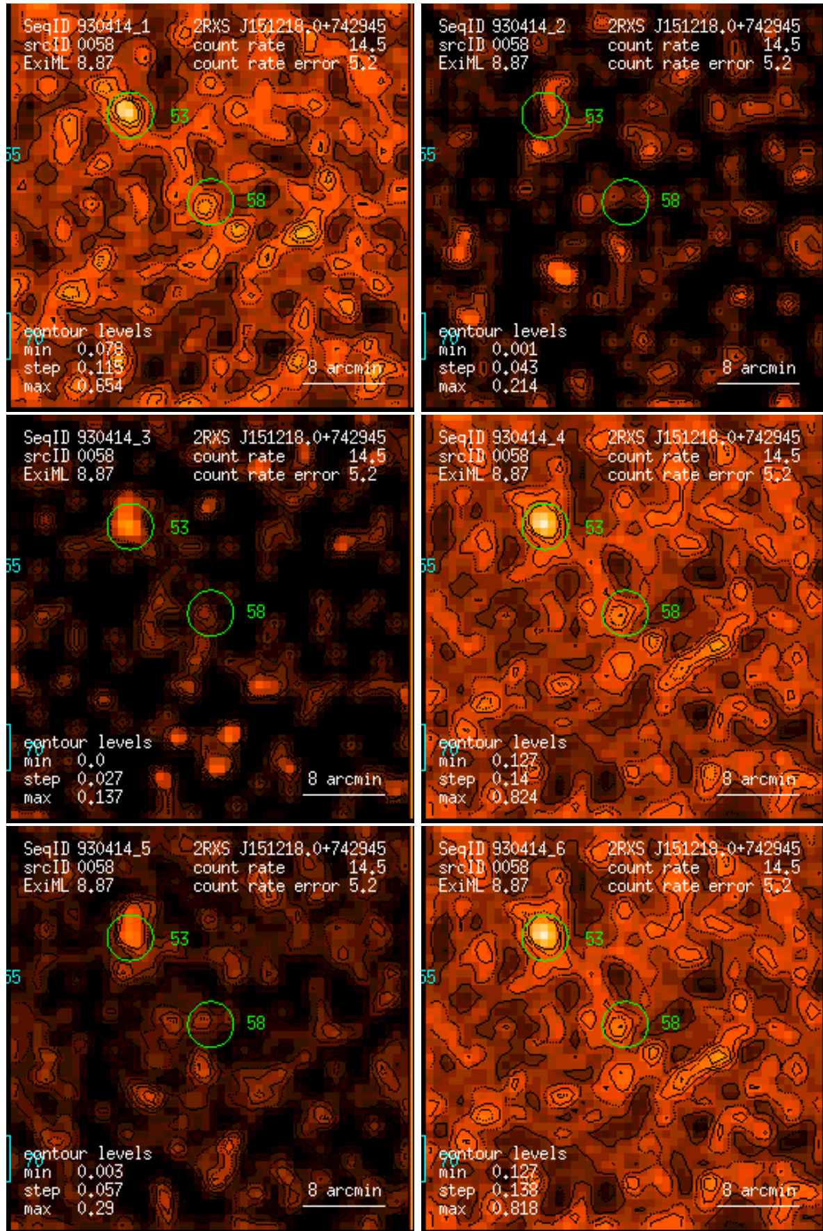
Figure 58: RASS 930414: detection 0058: band rate images, Gaussian filter: (1) PSPC channels 11 – 41, (2) 52 – 90, (3) 91 – 201, (4) 11 – 235, (5) 52 – 201, (6) 11 – 201. Broad band rates in counts/ks. Band rate contour levels in counts/ks/arcmin 2 .
