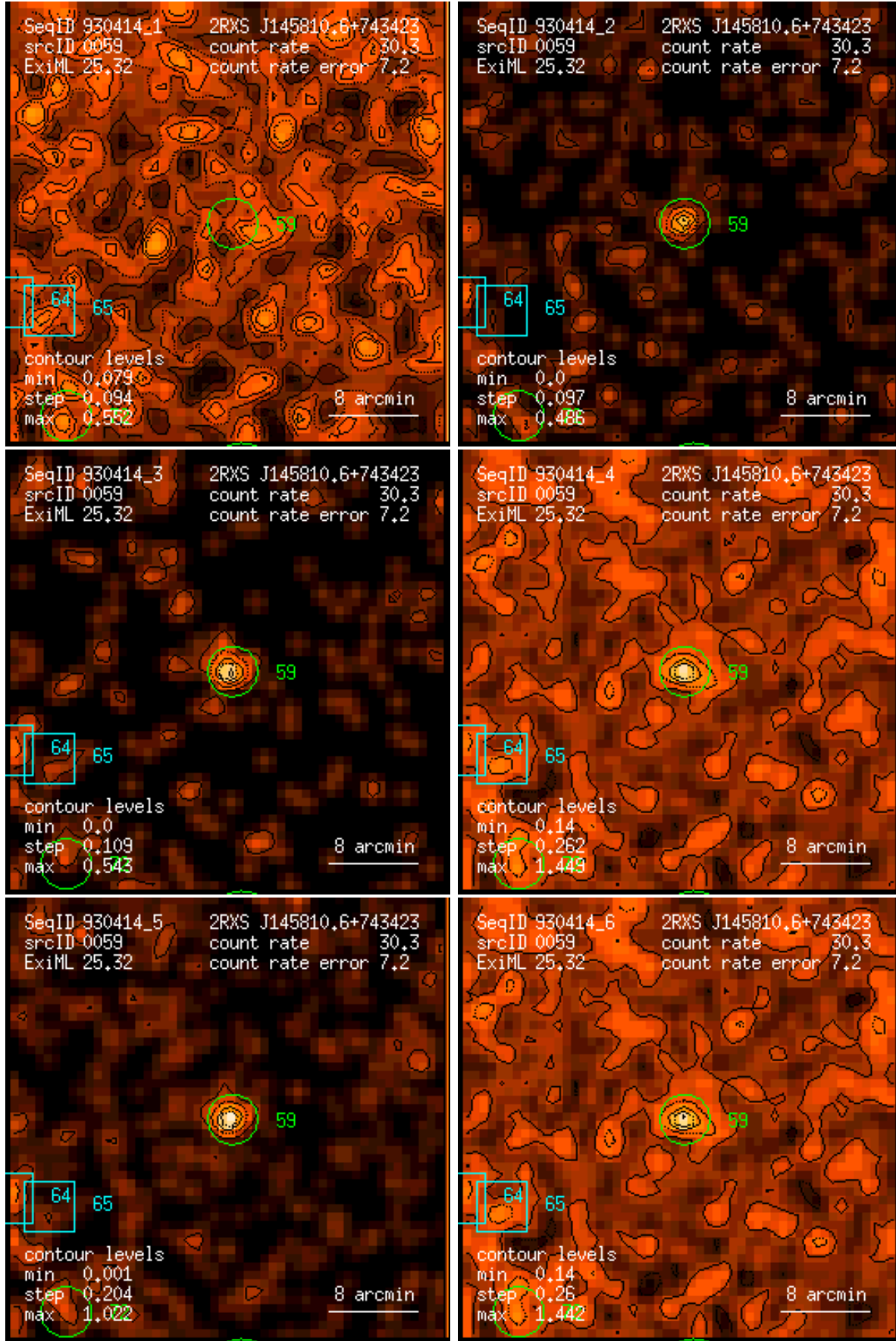
Figure 59: RASS 930414: detection 0059: band rate images, Gaussian filter: (1) PSPC channels 11 – 41, (2) 52 – 90, (3) 91 – 201, (4) 11 – 235, (5) 52 – 201, (6) 11 – 201. Broad band rates in counts/ks. Band rate contour levels in counts/ks/arcmin 2 .
