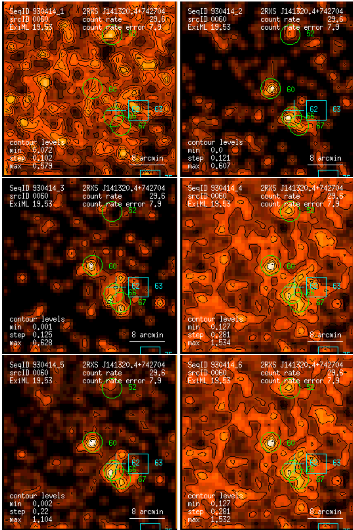
Figure 60: RASS 930414: detection 0060: band rate images, Gaussian filter: (1) PSPC channels 11 – 41, (2) 52 – 90, (3) 91 – 201, (4) 11 – 235, (5) 52 – 201, (6) 11 – 201. Broad band rates in counts/ks. Band rate contour levels in counts/ks/arcmin 2 .
