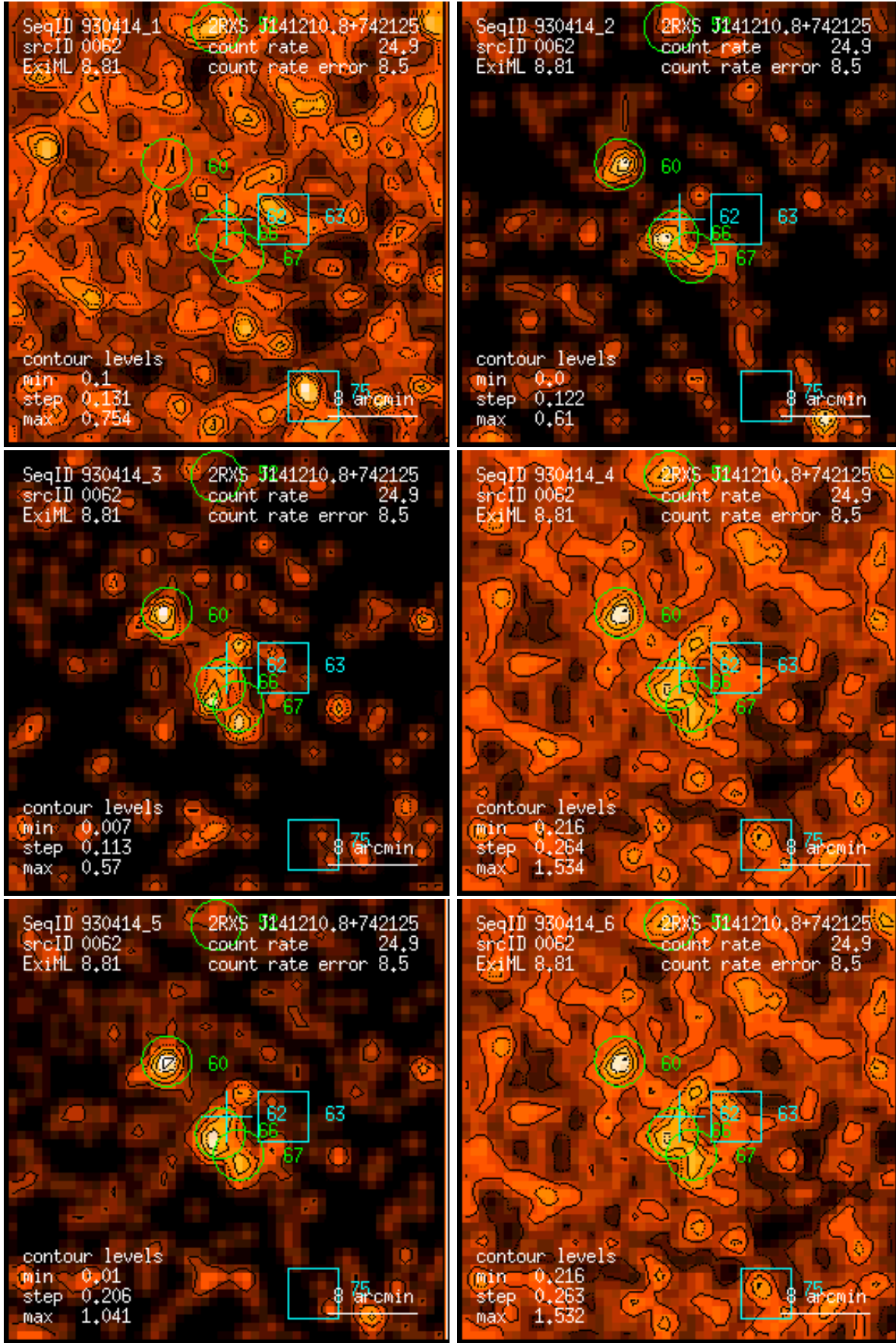
Figure 62: RASS 930414: detection 0062: band rate images, Gaussian filter: (1) PSPC channels 11 – 41, (2) 52 – 90, (3) 91 – 201, (4) 11 – 235, (5) 52 – 201, (6) 11 – 201. Broad band rates in counts/ks. Band rate contour levels in counts/ks/arcmin 2 .
