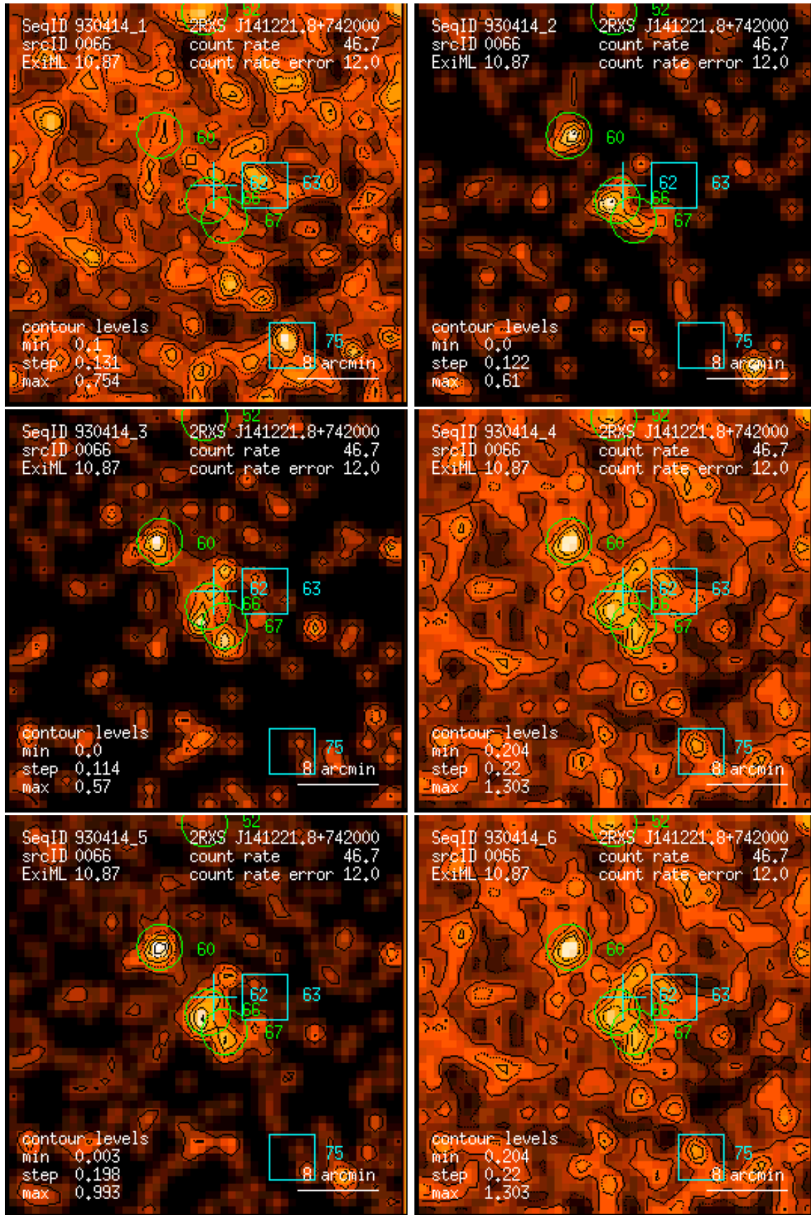
Figure 66: RASS 930414: detection 0066: band rate images, Gaussian filter: (1) PSPC channels 11 – 41, (2) 52 – 90, (3) 91 – 201, (4) 11 – 235, (5) 52 – 201, (6) 11 – 201. Broad band rates in counts/ks. Band rate contour levels in counts/ks/arcmin 2 .
