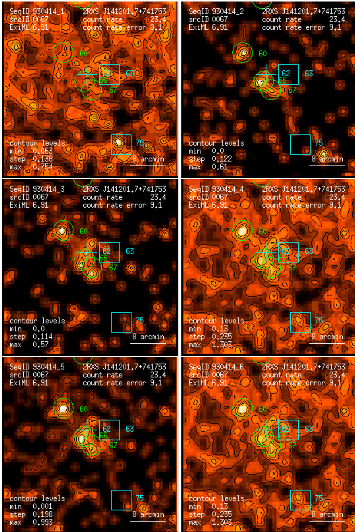
Figure 67: RASS 930414: detection 0067: band rate images, Gaussian filter: (1) PSPC channels 11 – 41, (2) 52 – 90, (3) 91 – 201, (4) 11 – 235, (5) 52 – 201, (6) 11 – 201. Broad band rates in counts/ks. Band rate contour levels in counts/ks/arcmin 2 .
