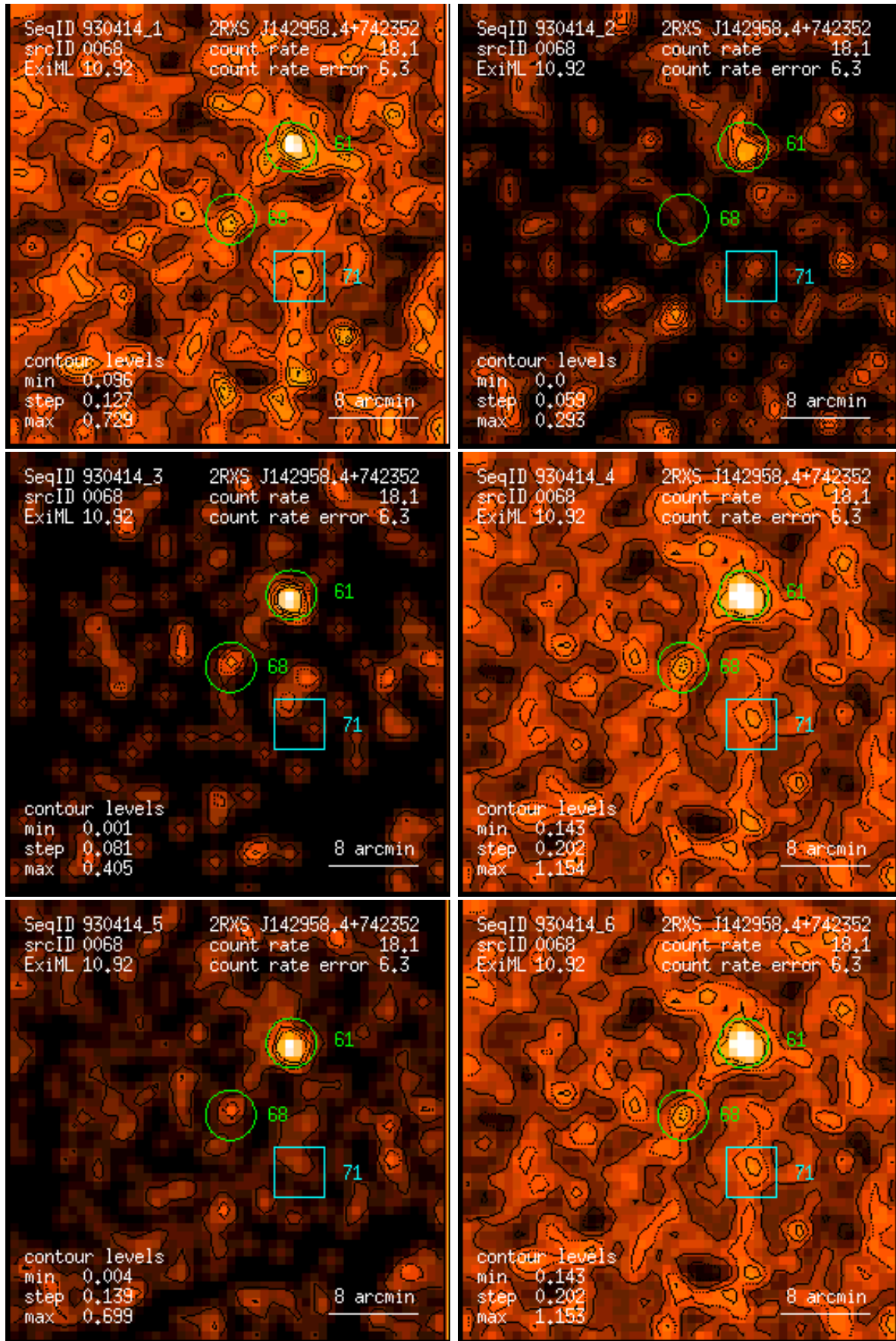
Figure 68: RASS 930414: detection 0068: band rate images, Gaussian filter: (1) PSPC channels 11 – 41, (2) 52 – 90, (3) 91 – 201, (4) 11 – 235, (5) 52 – 201, (6) 11 – 201. Broad band rates in counts/ks. Band rate contour levels in counts/ks/arcmin 2 .
