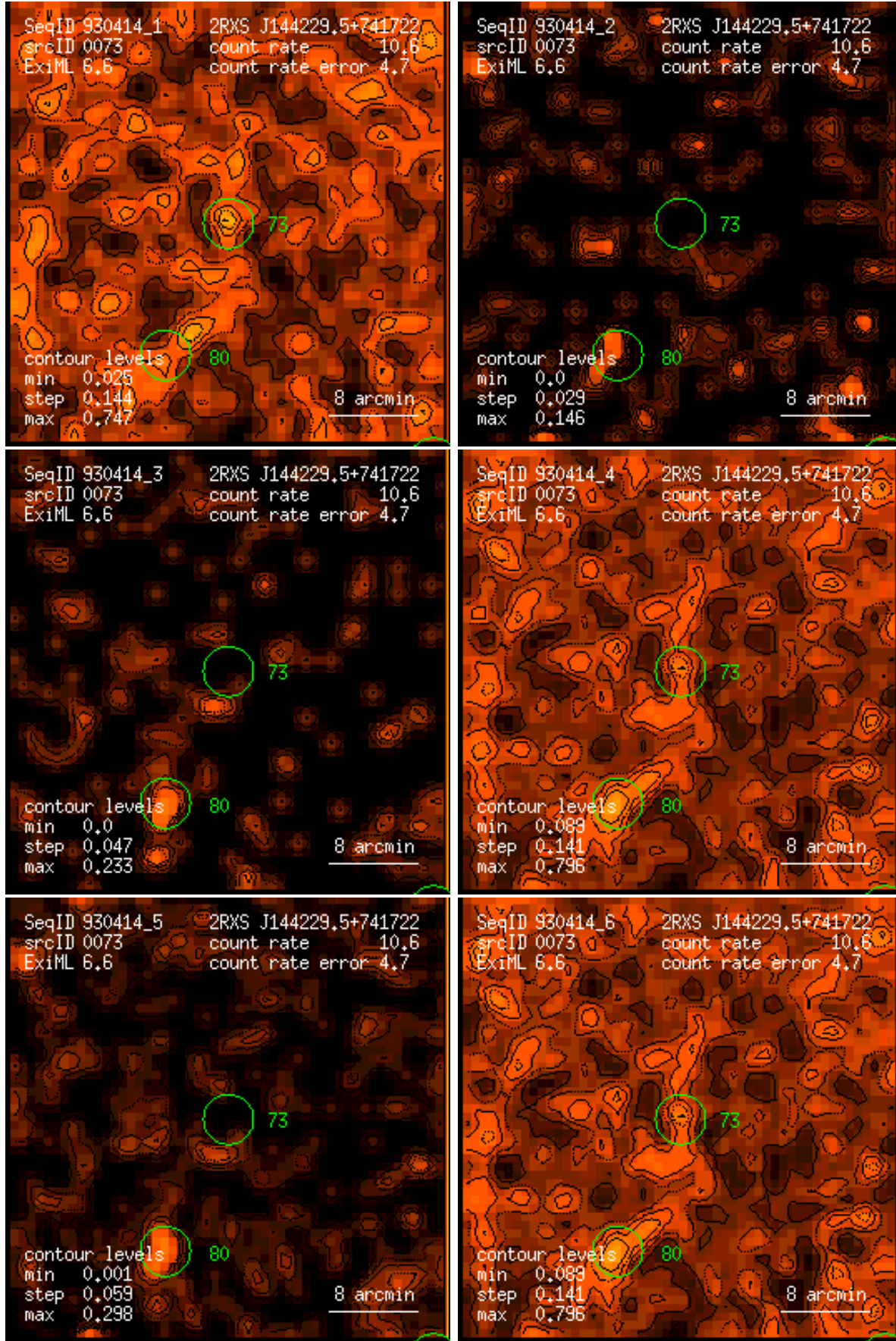
Figure 73: RASS 930414: detection 0073: band rate images, Gaussian filter: (1) PSPC channels 11 – 41, (2) 52 – 90, (3) 91 – 201, (4) 11 – 235, (5) 52 – 201, (6) 11 – 201. Broad band rates in counts/ks. Band rate contour levels in counts/ks/arcmin 2 .
