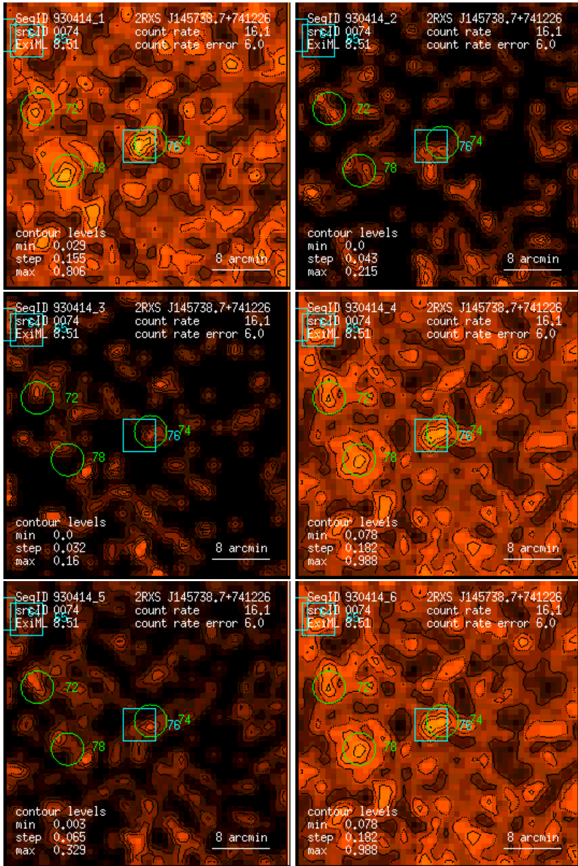
Figure 74: RASS 930414: detection 0074: band rate images, Gaussian filter: (1) PSPC channels 11 – 41, (2) 52 – 90, (3) 91 – 201, (4) 11 – 235, (5) 52 – 201, (6) 11 – 201. Broad band rates in counts/ks. Band rate contour levels in counts/ks/arcmin 2 .
